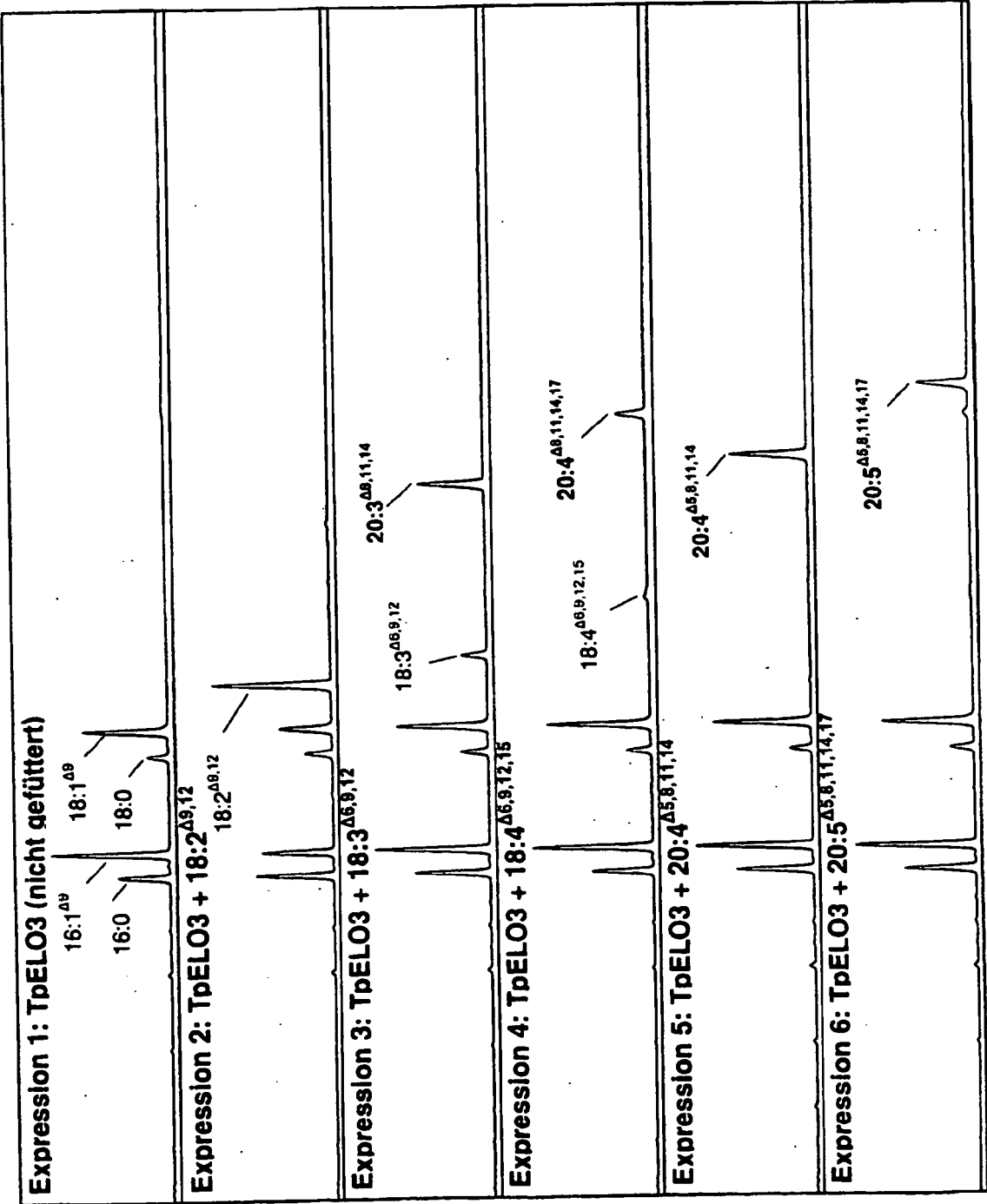
Figur 10: Expression von TpELO3 in Hefe.
