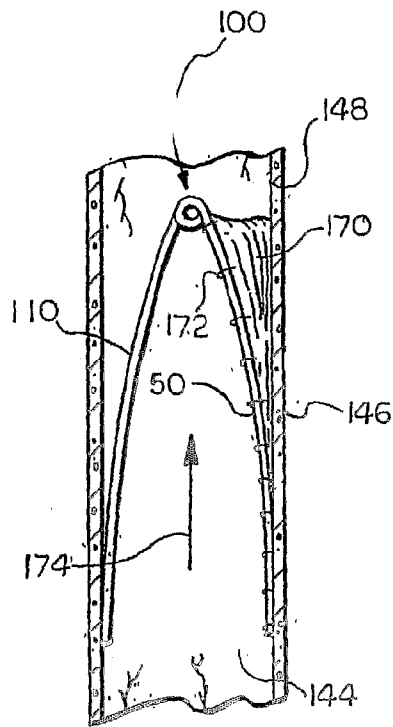
FIG. 3 (PRIOR ART)
