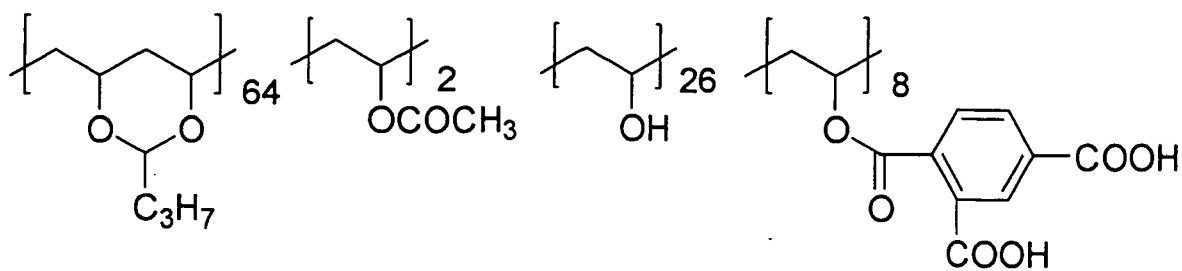
Binder polymer (2)
