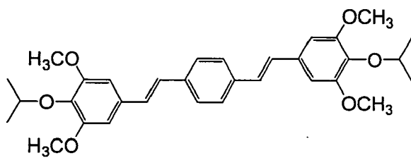
Sensitizing dye (2)
