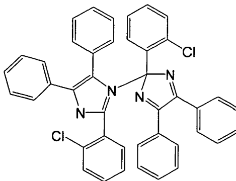
Polymerization initiator ( 1 )
