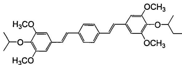
Sensitizing dye (3)
