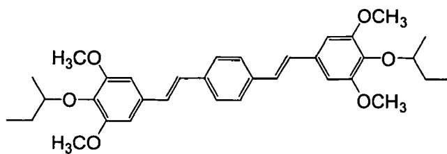
Sensitizing dye (1)
