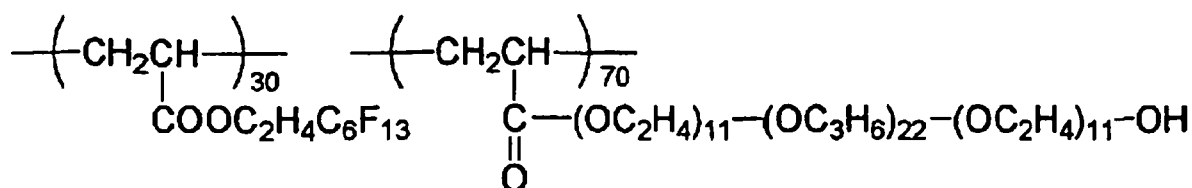
Water-soluble fluorine-based surfactant ( 1 )
