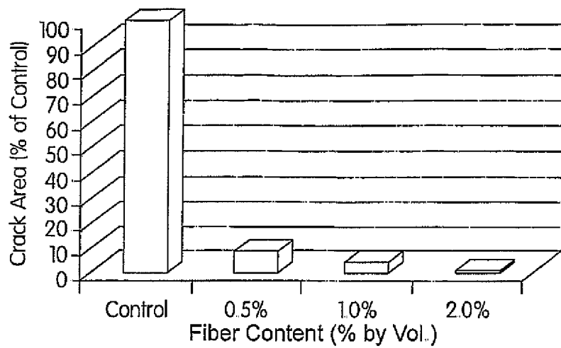
Comparison of Crack Areas as a Percentage of Control for Different Fiber Contents
