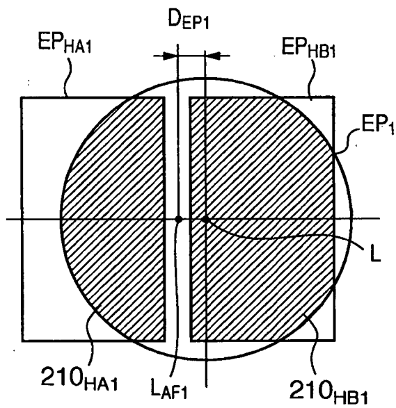
TELEPHOTO END
