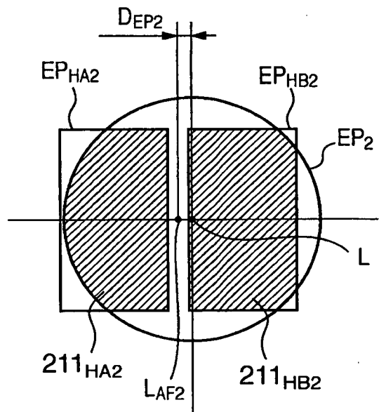
WIDE-ANGLE END
