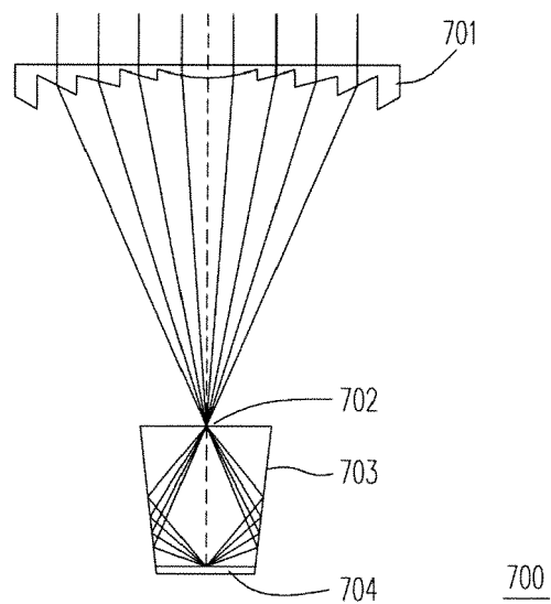
FIG. 7 (RELATED ART)
