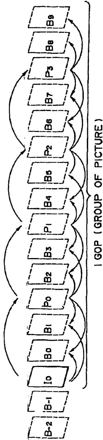
FIG. 8A STRUCTURE FOR INTERFRAME PREDICTION
