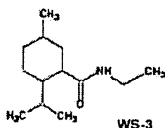
N-ethyl-p-menthane-3-carboxamide
