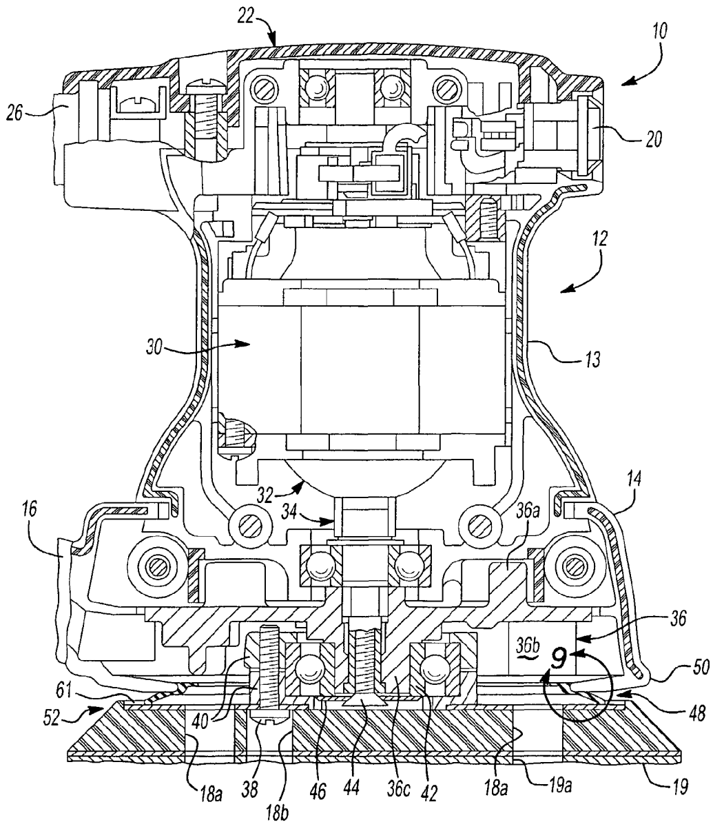
Fig-8 PRIOR ART
