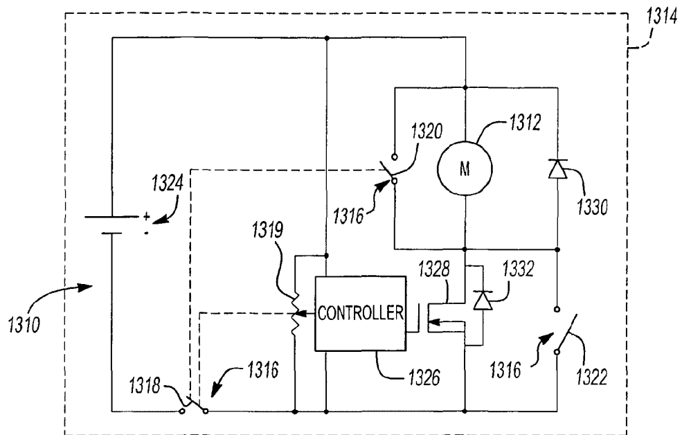
Fig-13 PRIOR ART
