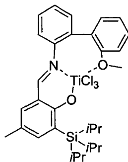
Compound 30
