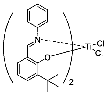
Compound 46
