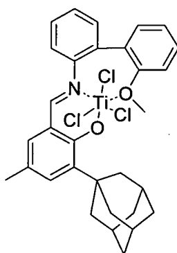
Compound 9
