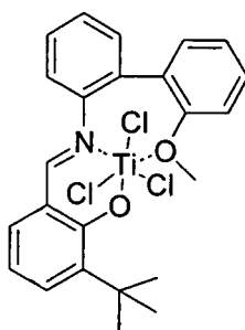
Compound 14
