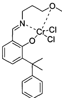
Compound 44
