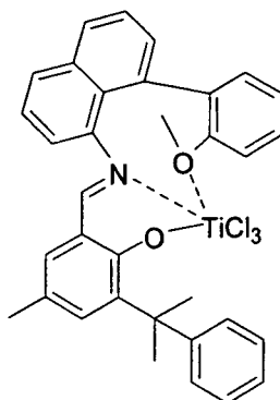
Compound 13
