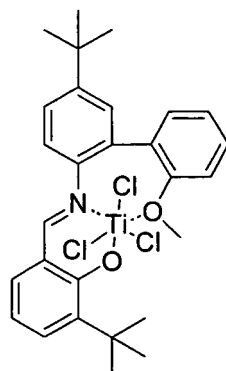
Compound 35
