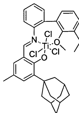
Compound 33
