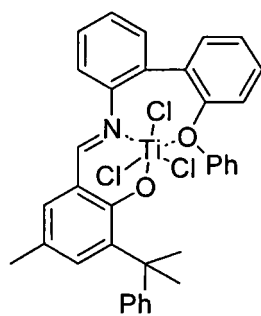
Compound 37
