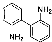
Compound 39
