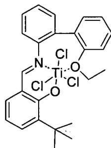
Compound 22
