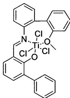
Compound 32
