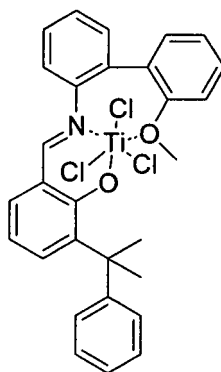
Compound 5
