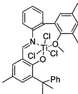
Compound 24
