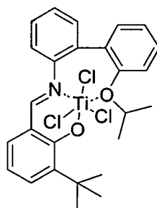
Compound 20
