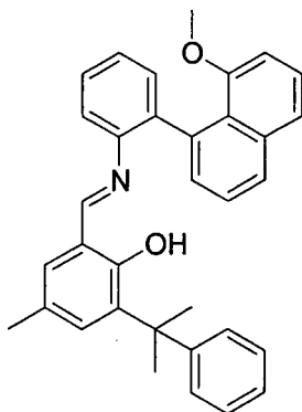
Compound 10
