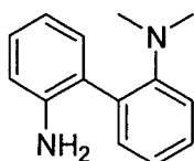
Compound 41
