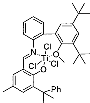
Compound 21
