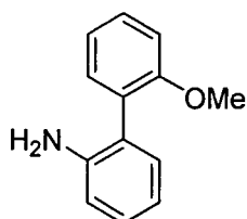
Compound 3
