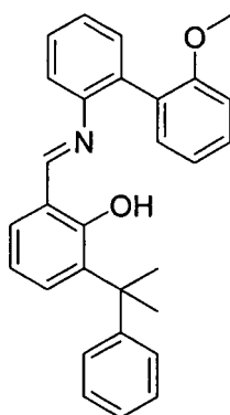
Compound 4
