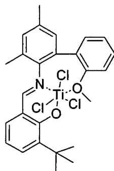
Compound 19
