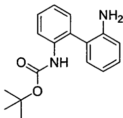
Compound 40
