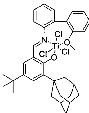
Compound 27
