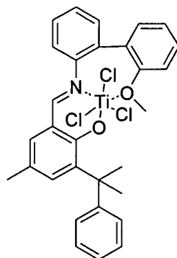
Compound 7
