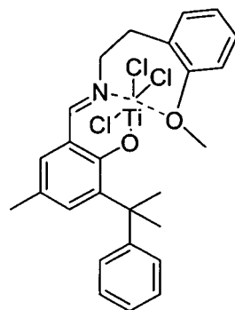
Compound 38
