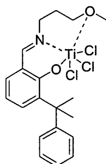
Compound 2
