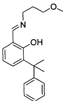
Compound 1
