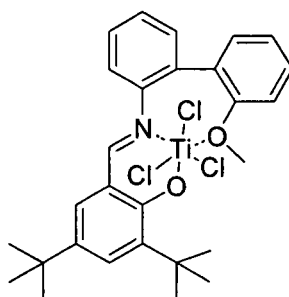
Compound 17
