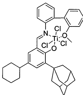
Compound 26
