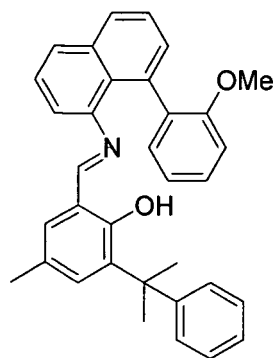
Compound 12
