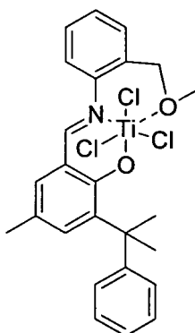
Compound 36
