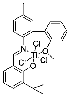
Compound 18
