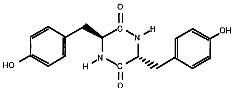
Chemical Formula (8)
