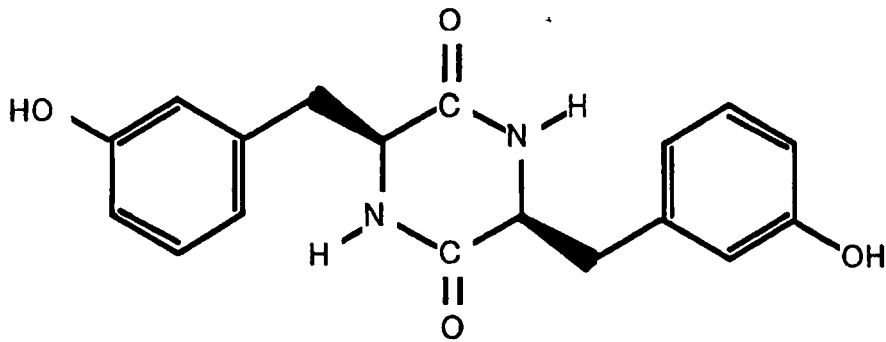
Chemical Formula (13)
