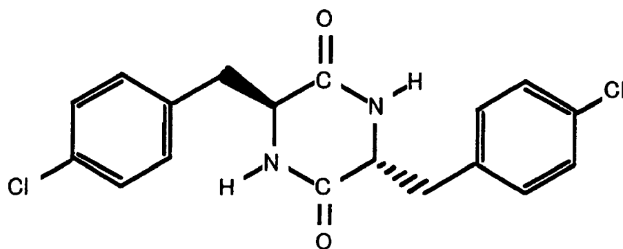
Chemical Formula (11)
