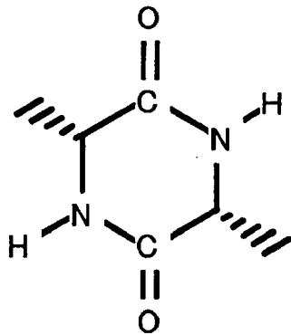
Chemical Formula (3)
