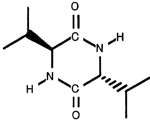
Anhydride DL-Valine
