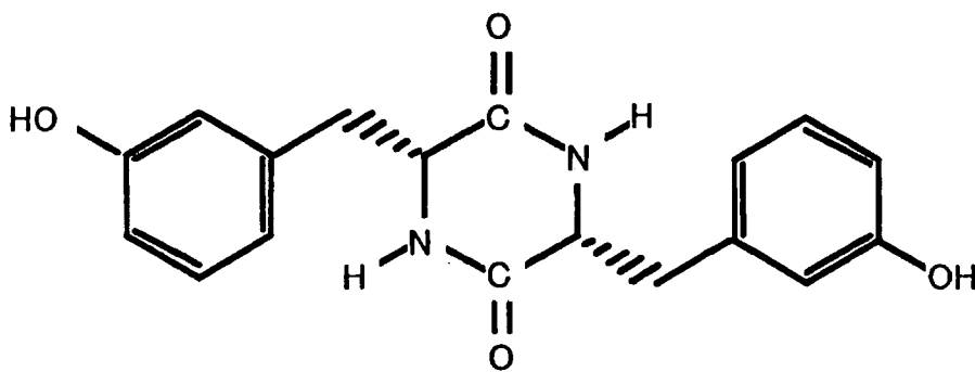
Chemical Formula (15)
