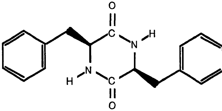
Anhydride L-Phenylalanine
