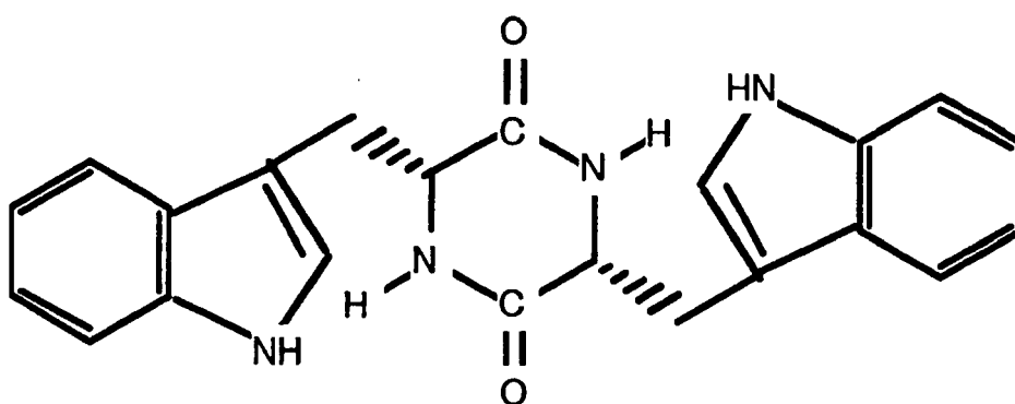
Chemical Formula (26)
