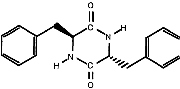
Anhydride DL-Phenylalanine
