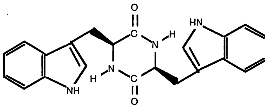
Chemical Formula (24)
