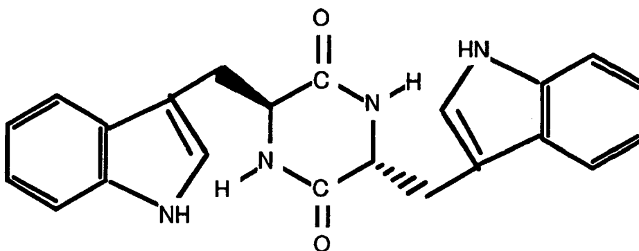
Chemical Formula (25)
