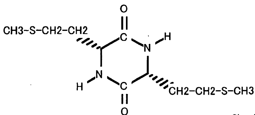
Chemical Formula (20)
