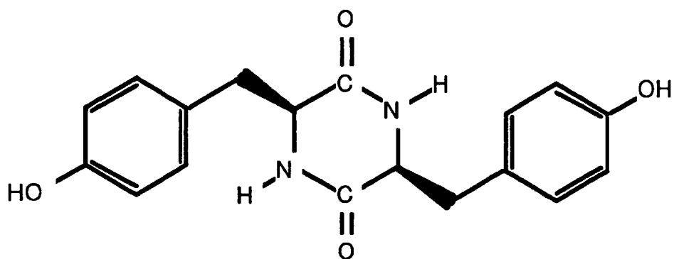
Chemical Formula (7)
