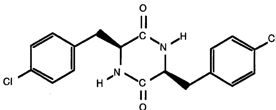
Anhydride L-p-Chlorophenylalanine
