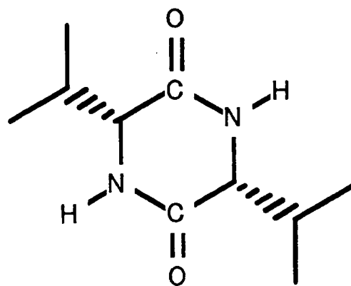
Anhydride D-Valine
