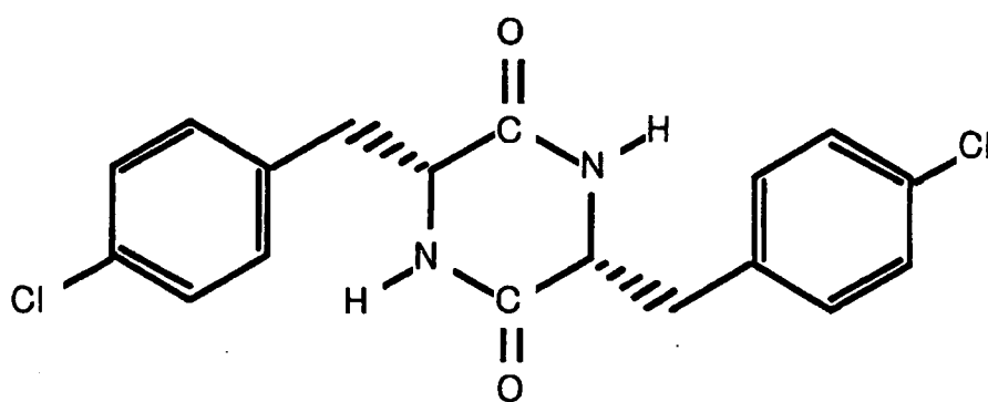
Anhydride D-p-Chlorophenylalanine
