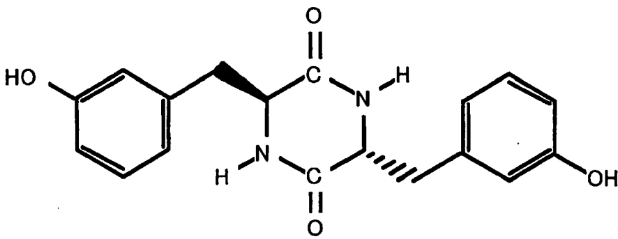
Chemical Formula (14)
