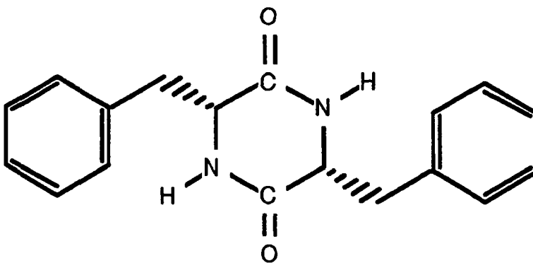
Anhydride D-Phenylalanine
