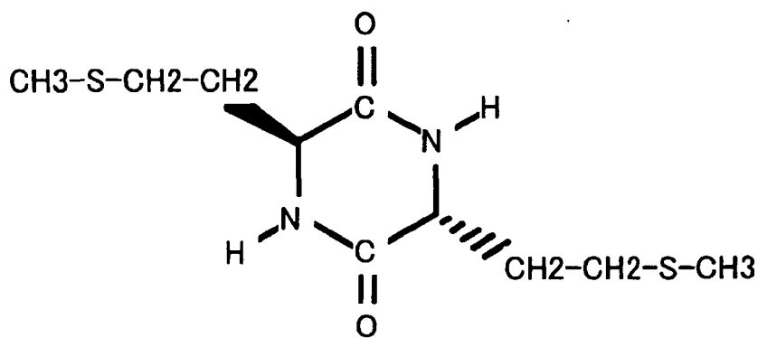
Chemical Formula (19)
