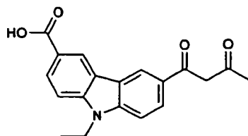
Compound No.8
