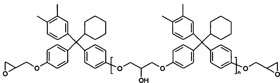
Compound No.16
