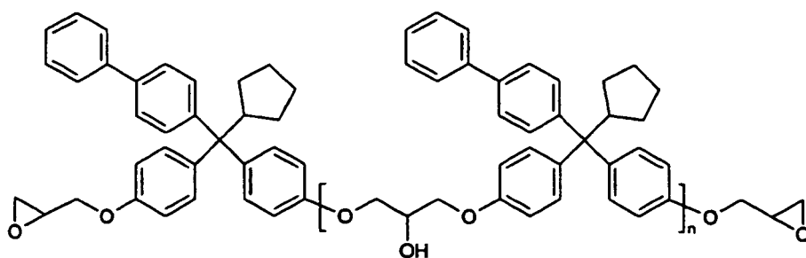
Compound No.18
