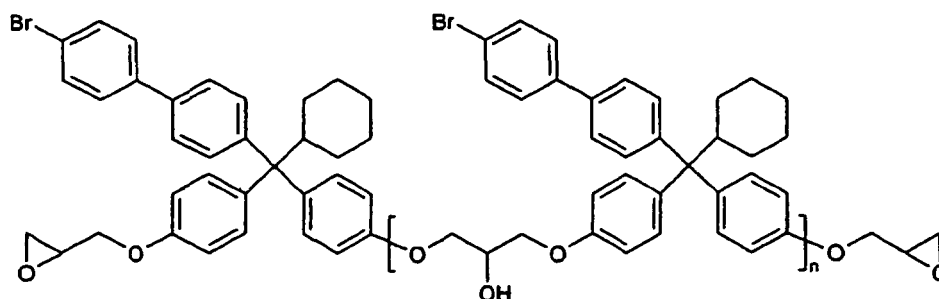
Compound No.20
