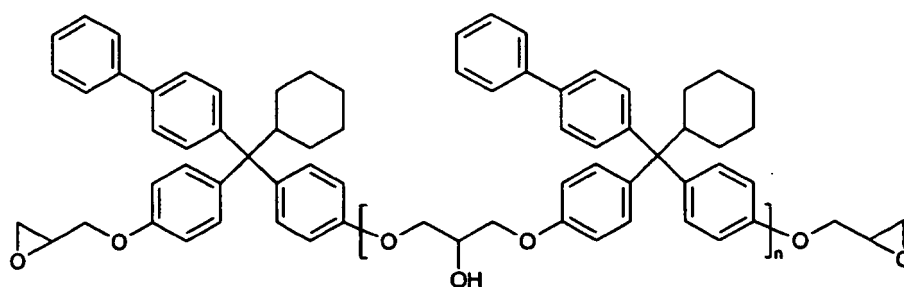
Compound No.12
