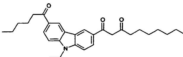
Compound No.9
