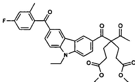
Compound No.24
