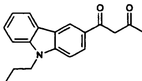
Compound No.1
