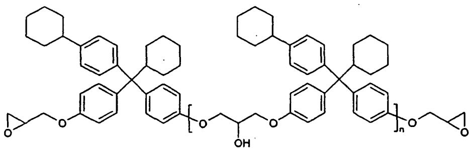
Compound No.19
