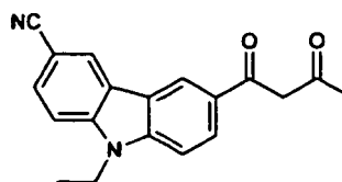
Compound No.7
