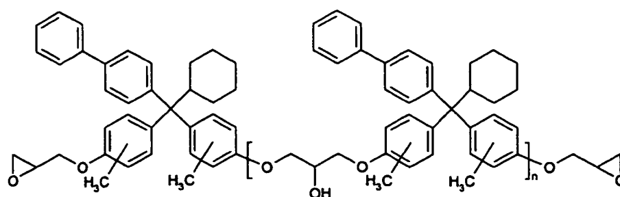
Compound No.13
