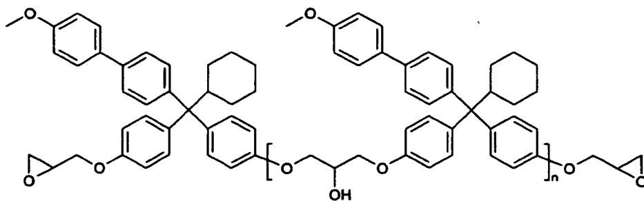
Compound No.17
