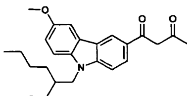
Compound No.10
