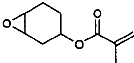
Compound No.29
