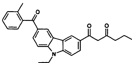
Compound No.4
