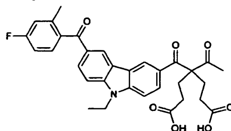
Compound No.25
