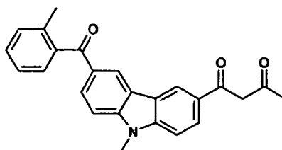
Compound No.3
