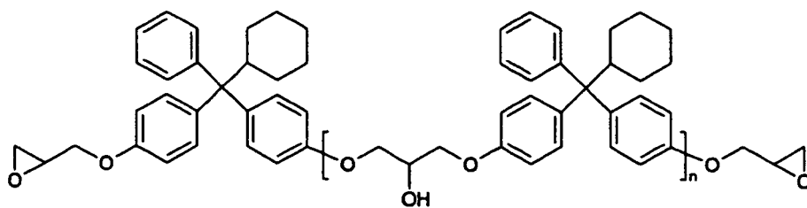
Compound No.15
