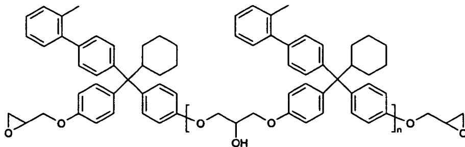
Compound No.14
