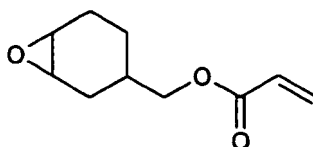
Compound No.30
