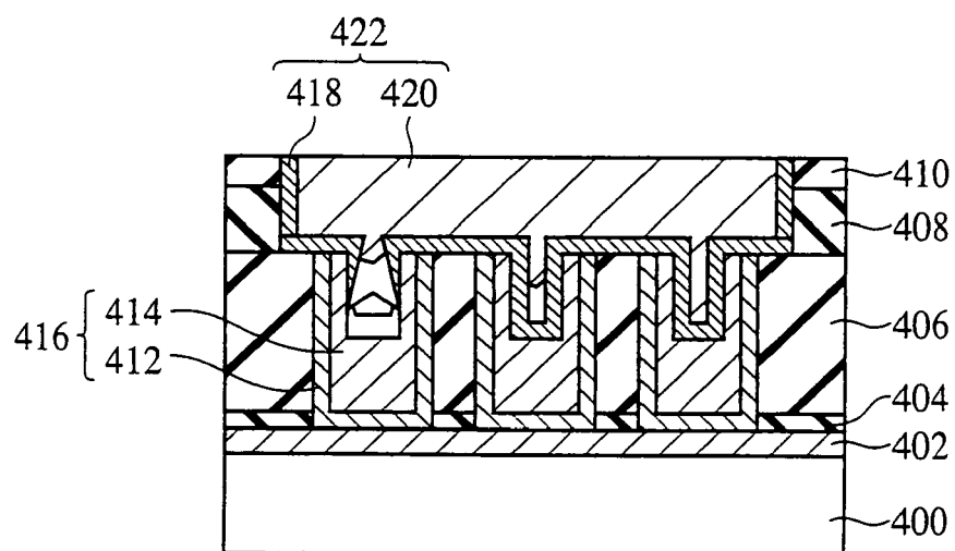
FIG. 38 PRIOR ART
