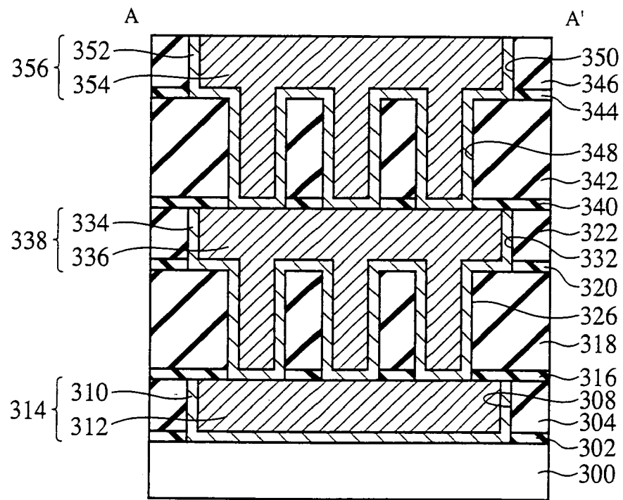
FIG. 36 PRIOR ART
