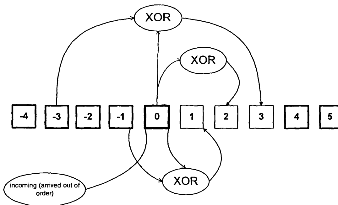
Offset based 1-Packet Recovery Schema 2
