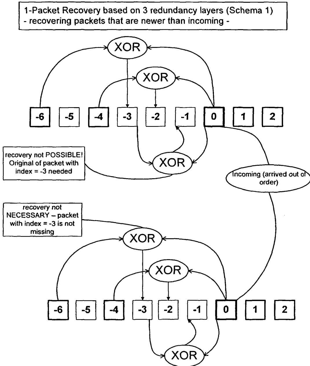
Offset based 1-Packet Recovery Schema 1
