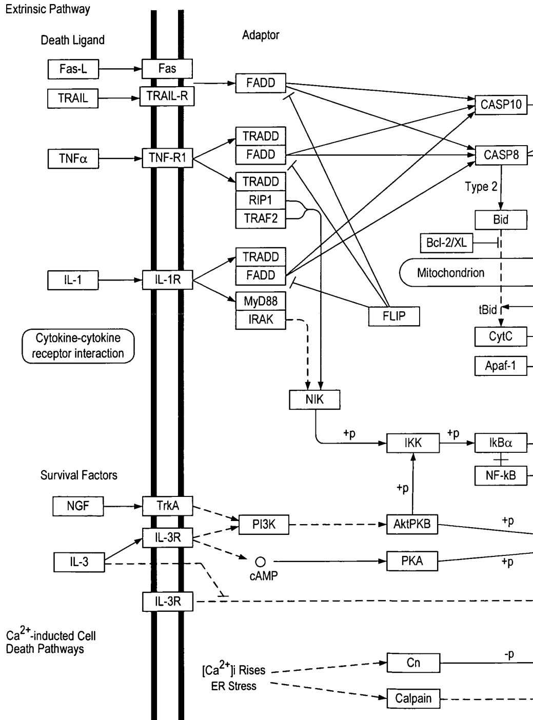
Fig. 3G APOPTOSIS
