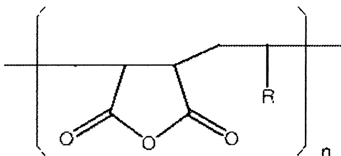
Structural Formula (1)
