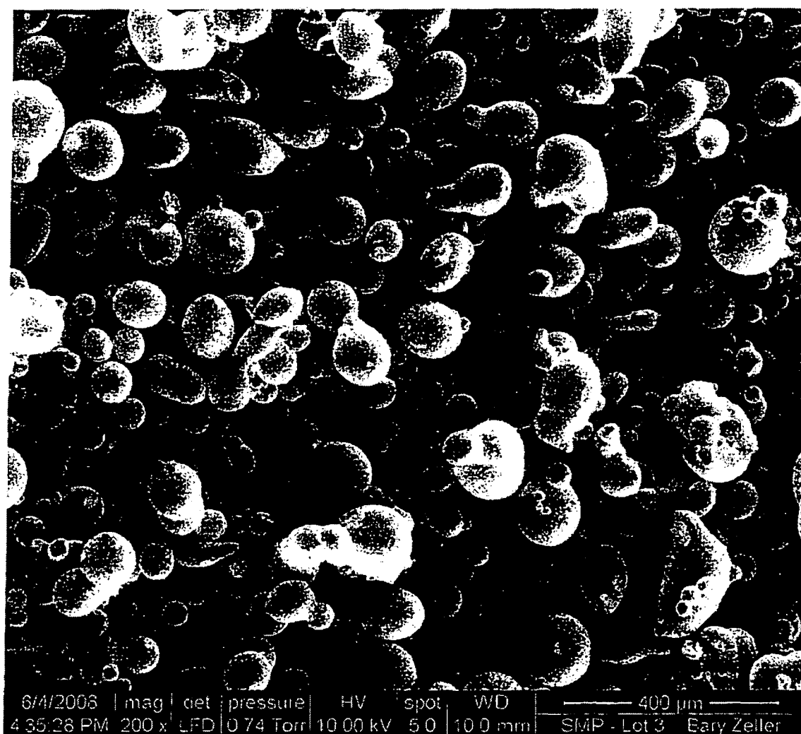
FIG. 4A: Particulate Ingredient at 200x Magnification
