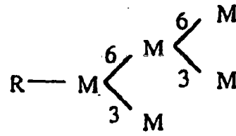
M_5 . High-mannose
