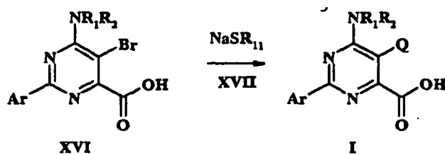
Scheme 8
