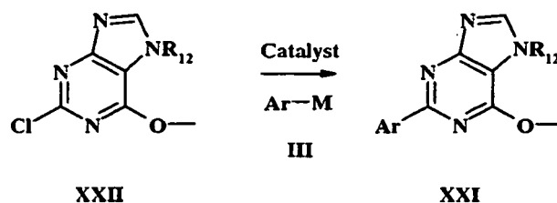
Scheme 12
