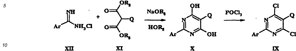
Scheme 5
