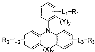
Chemical Formula 1
