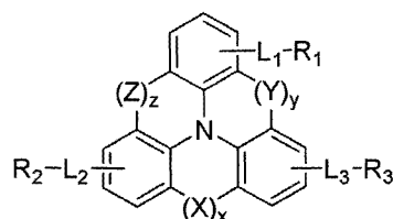
Chemical Formula 2
