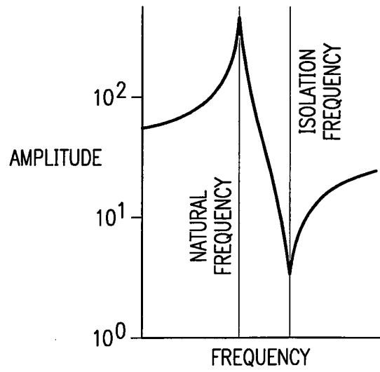
FIG. 4C (PRIOR ART)
