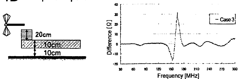
FIG. 14D Example of impedance difference in third case
