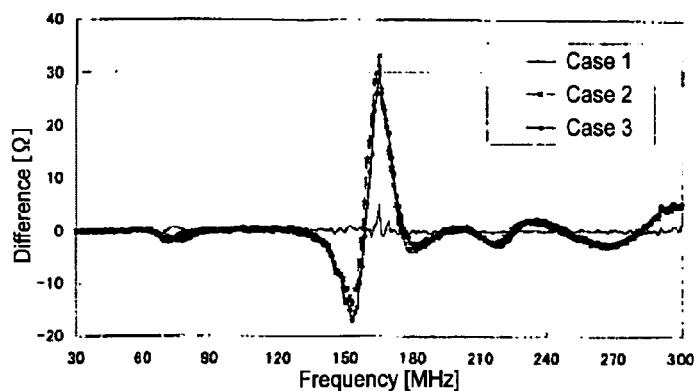
FIG. 14B Example of impedance difference in first case
