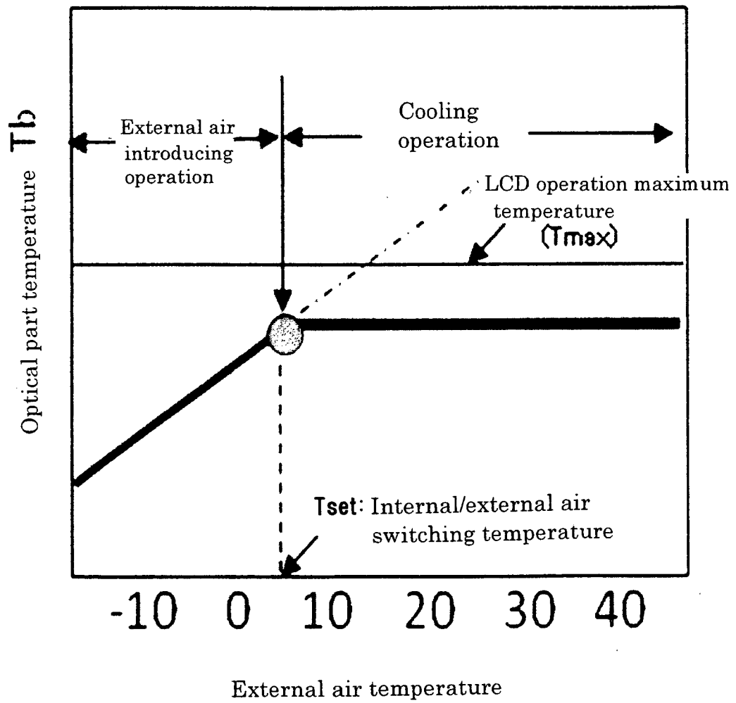
Relation between external air temperature and optical part temperature
