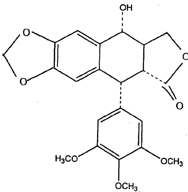
Podophyllotoxin
