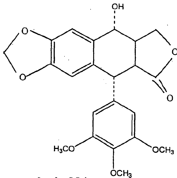
Picropodophyllin
