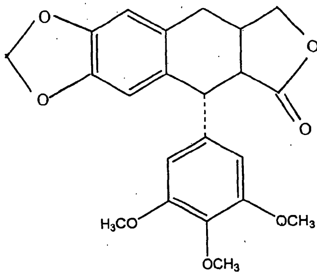
Deoxypicropodophyllin
