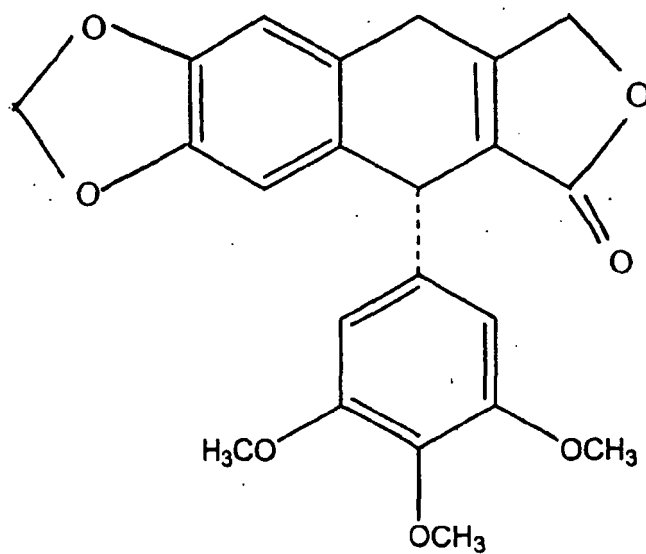
β-apopicropodophyllin
