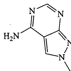
N 8 -8aza-7deazaadenine
