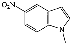
5-Nitroindole
