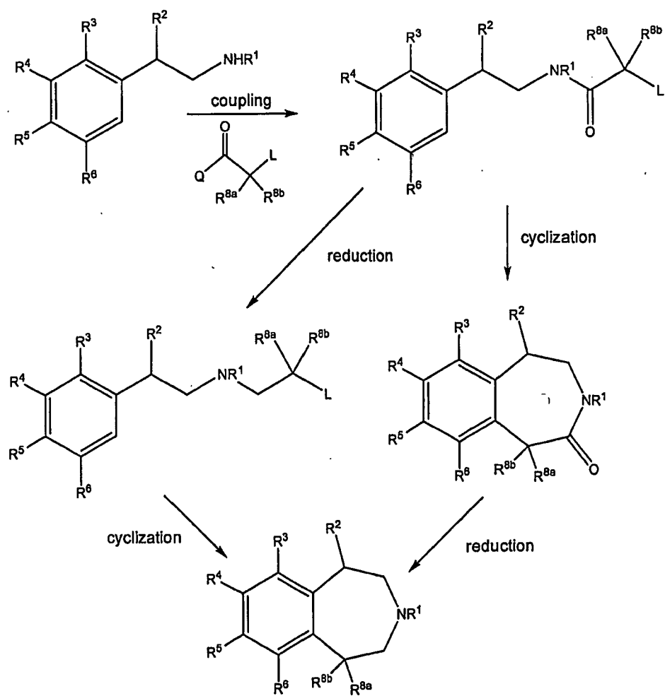
Scheme Ia
