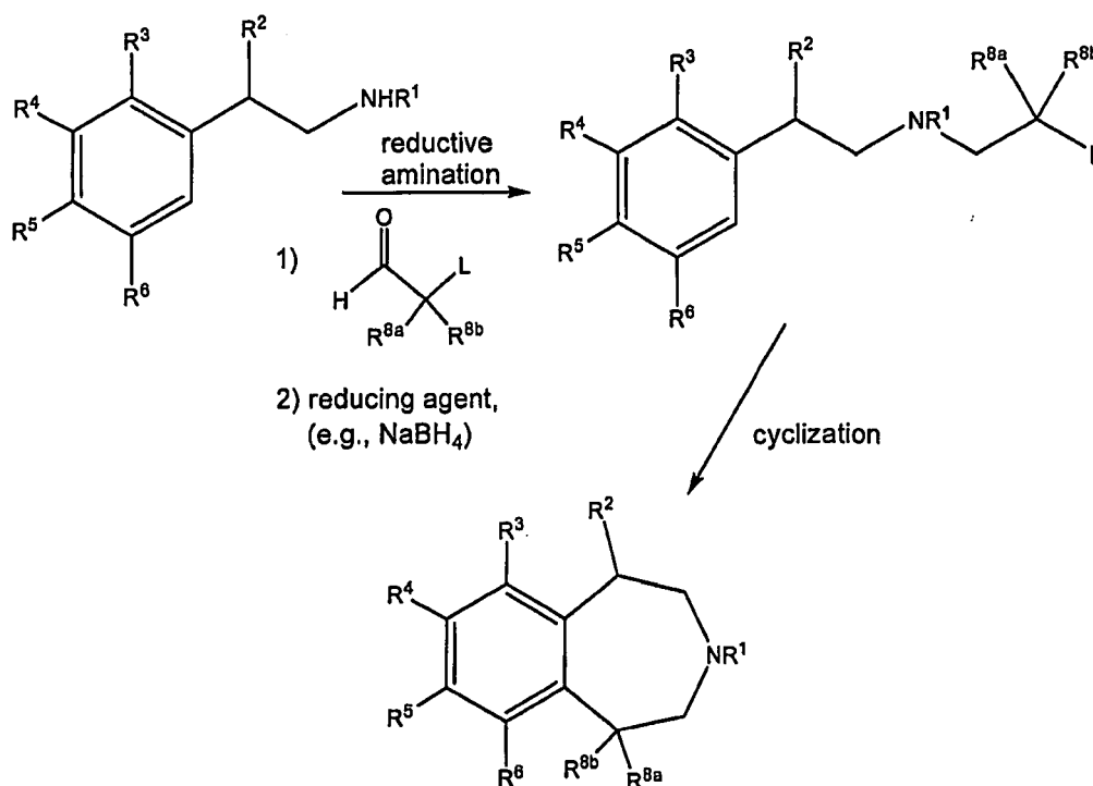
Scheme 1c
