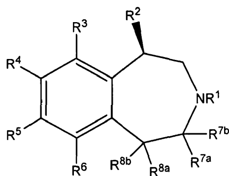
Ib
