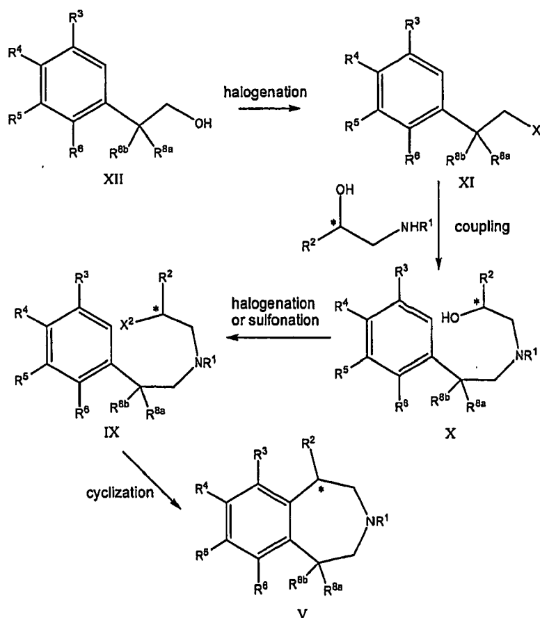
Scheme II
