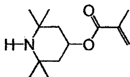
ADK STAB LA-87
