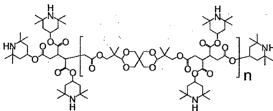
ADK STAB LA-68
