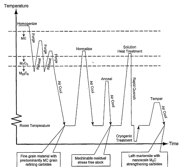
FIG. 2B A DIAGRAM OF THE TYPICAL PROCESSING PATH FOR ALLOYS OF THE INVENTION IN RELATION TO THE EQUILIBRIUM PHASES PRESENT.
