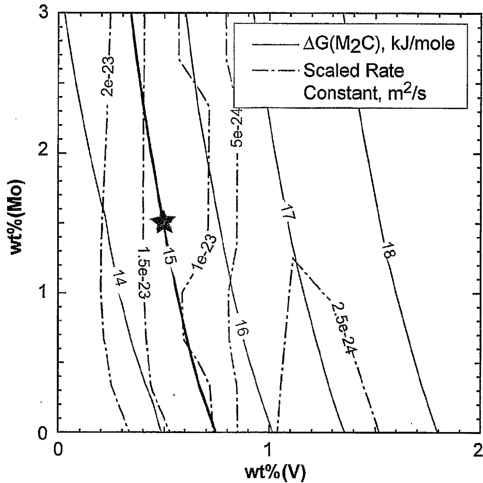
FIG. 4 CONTOURS OF M_2C DRIVING FORCE ( \Delta G ) AND SCALED RATE CONSTANT FOR VARYING MOLBDENUM ( Mo ) AND VANADIUM ( V ) CONTENTS, WHERE TEMPERATURE HAS BEEN SET TO 482^\circ C , AND AMOUNTS OF OTHER ALLOYING ELEMENTS HAVE BEEN SET TO, BY WEIGHT, 0.14% C, 9% Cr, 13% Co, AND 4.8% Ni.
