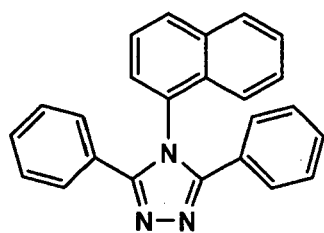
TAZ
