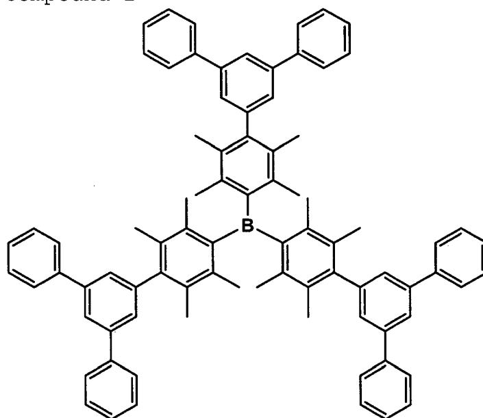
Compound 2
