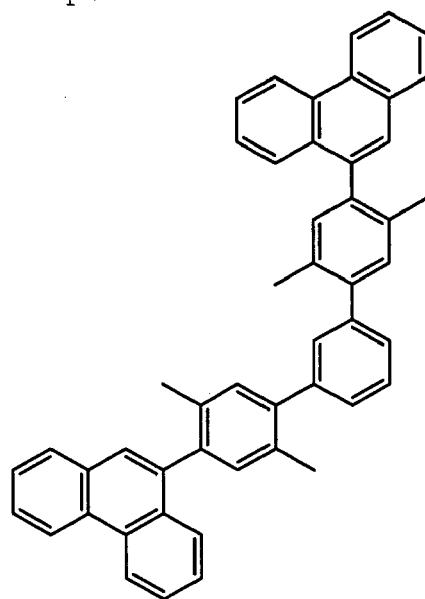
Compound 1
