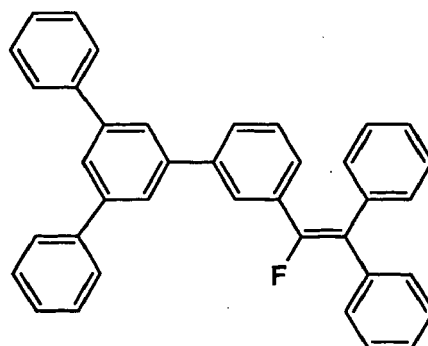
Compound 5
