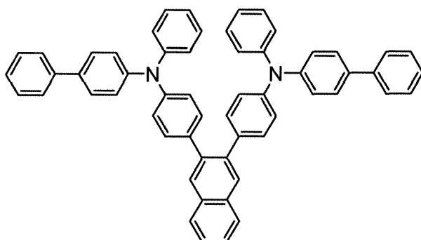
[Chemical Formula 5]
