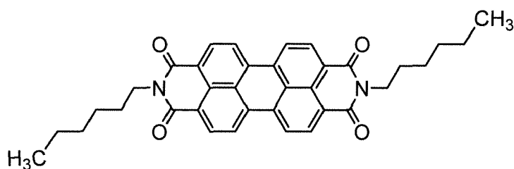
HexPTC
