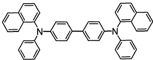
NPB
