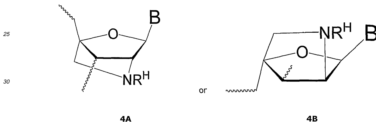
Scheme 4
