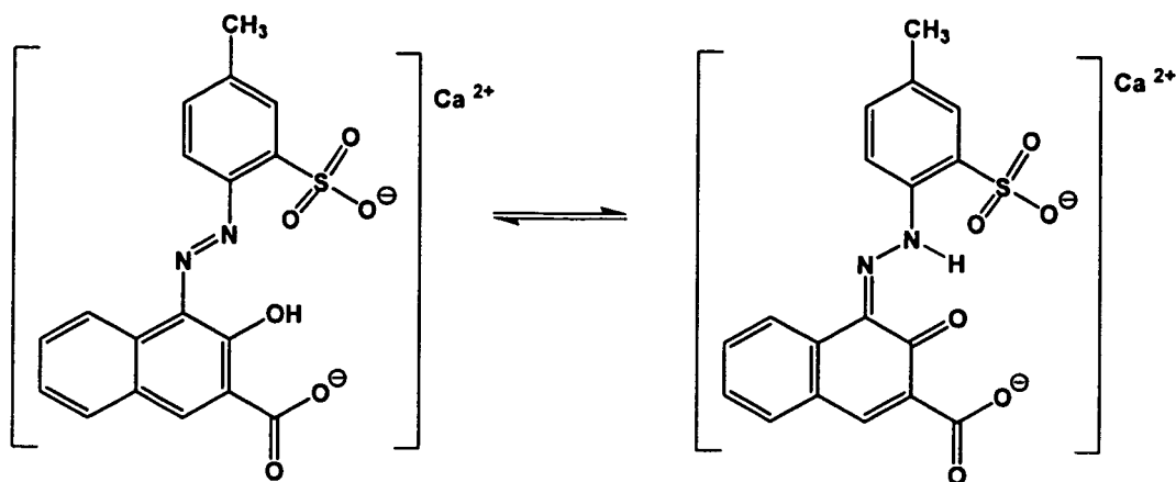
Enol-Azo tautomer
