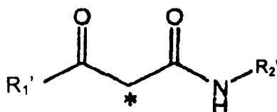
Formula (8)
