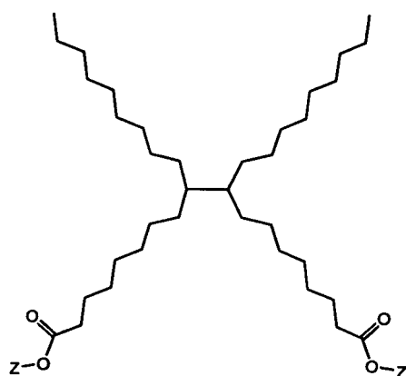
C36 Dimer Diacid
