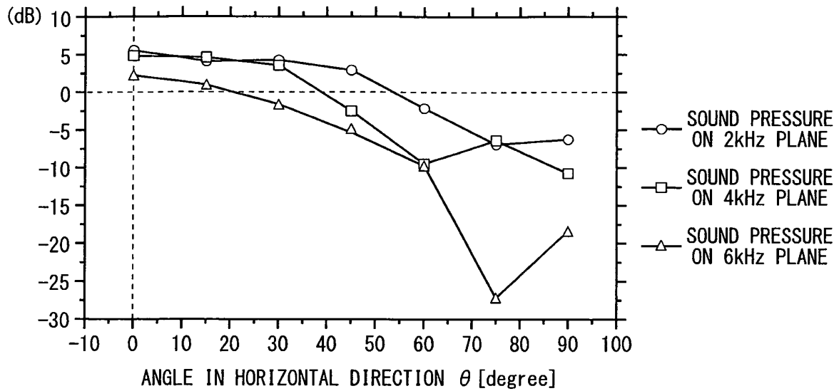
a CHANGE OF SOUND PRESSURE BY INCLINATION ANGLE IN HORIZONTAL DIRECTION FROM ON AXIS OF OPENING SURFACE
