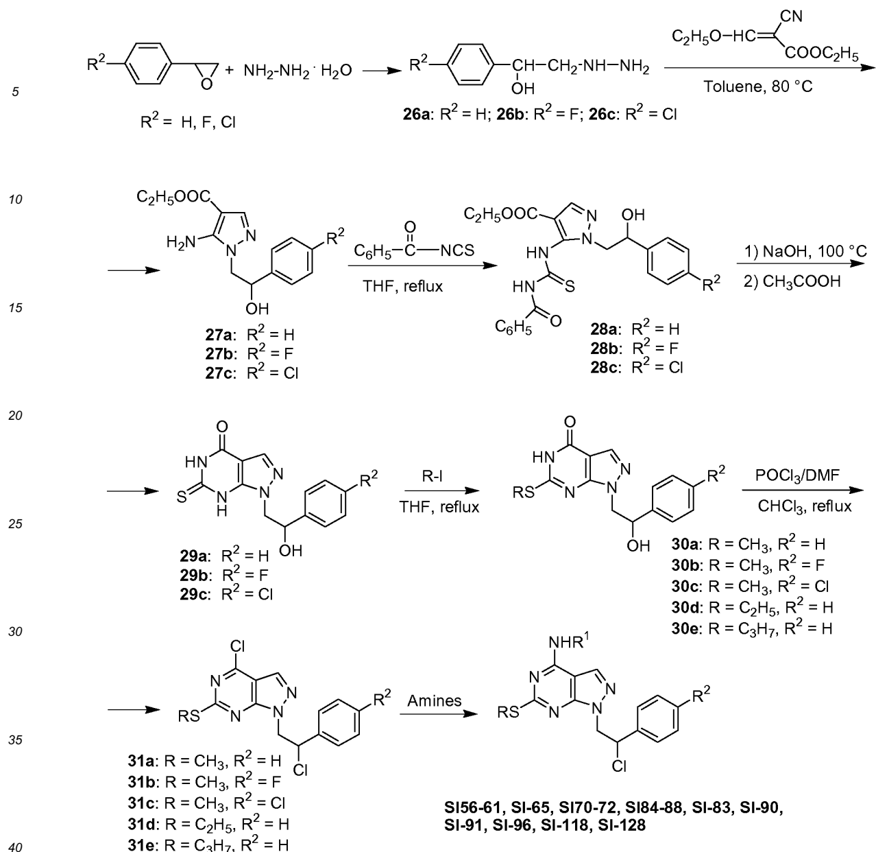
Scheme 1. Synthetic pathway to compounds SI56-61, SI-65, SI70-72, SI84-88, SI-83, SI-90, SI-91, SI-96, SI-118, SI-128.
