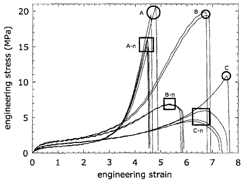
High Speed Tensile Results: Three Films
