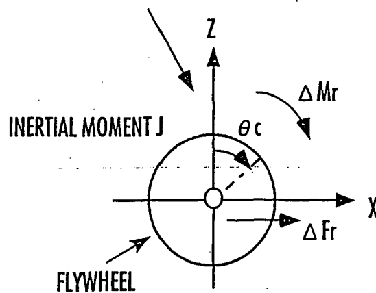
FIG.68 BODY POSTURE ANGLE CORRECTING PERTURBATION MODEL
