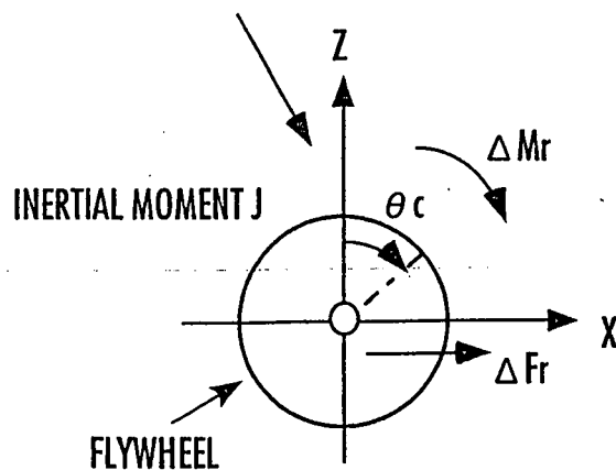
FIG.68 BODY POSTURE ANGLE CORRECTING PERTURBATION MODEL
