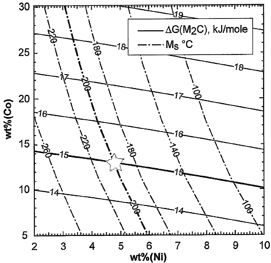
FIG. 6 CONTOURS OF M_s TEMPERATURE AND M_2C DRIVING FORCE ( \Delta G ) FOR VARYING COBALT (Co) AND NICKEL (Ni) CONTENTS, WHERE TEMPERATURE HAS BEEN SET TO 482°C, AND OTHER ALLOYING ELEMENT AMOUNTS HAVE BEEN SET TO, BY WEIGHT, 0.14% C, 9% Cr, 1.5% Mo, AND 0.5% V.
