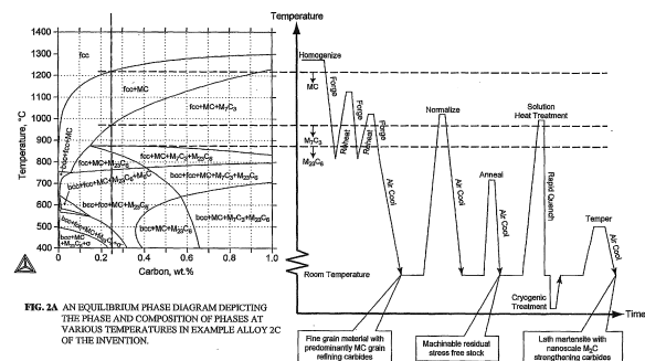
FIG. 2B A DIAGRAM OF THE TYPICAL PROCESSING PATH FOR ALLOYS OF THE INVENTION IN RELATION TO THE EQUILIBRIUM PHASES PRESENT.
