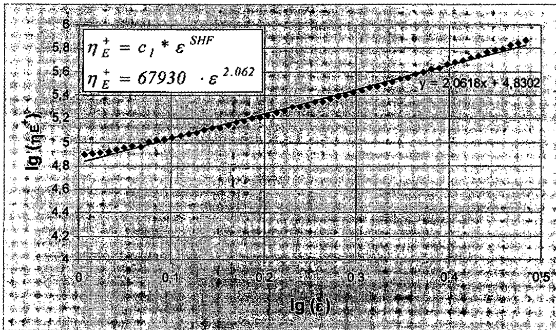
Figure 1: Determination of the SHI of WB130HMS at a strain rate of 0.1\text{s}^{-1} ^1 (SHI@ 0.1\text{s}^{-1} )
