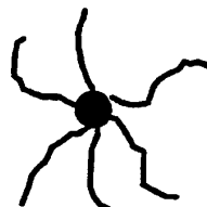
Star-branched
