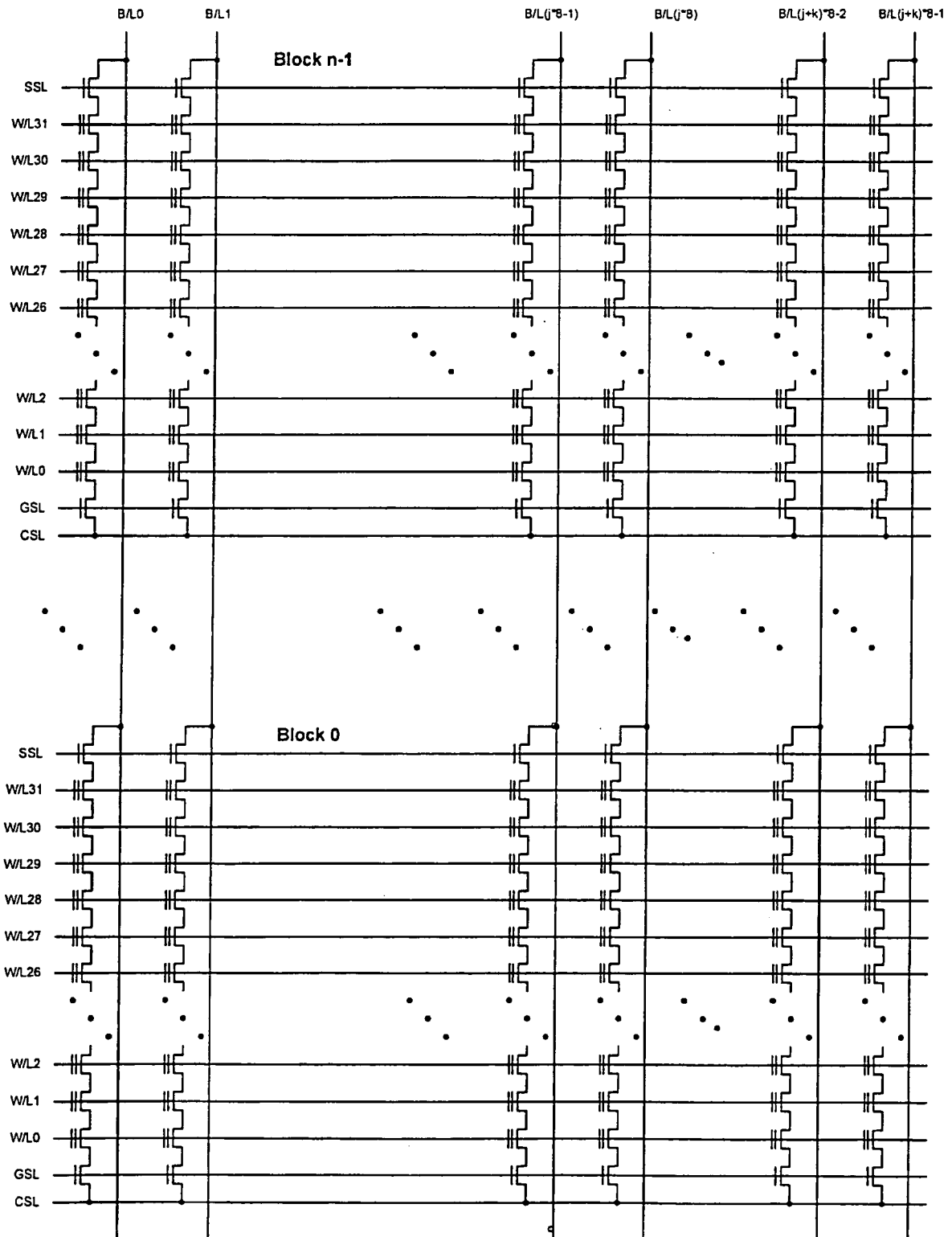
Fig. 9 Prior Art
