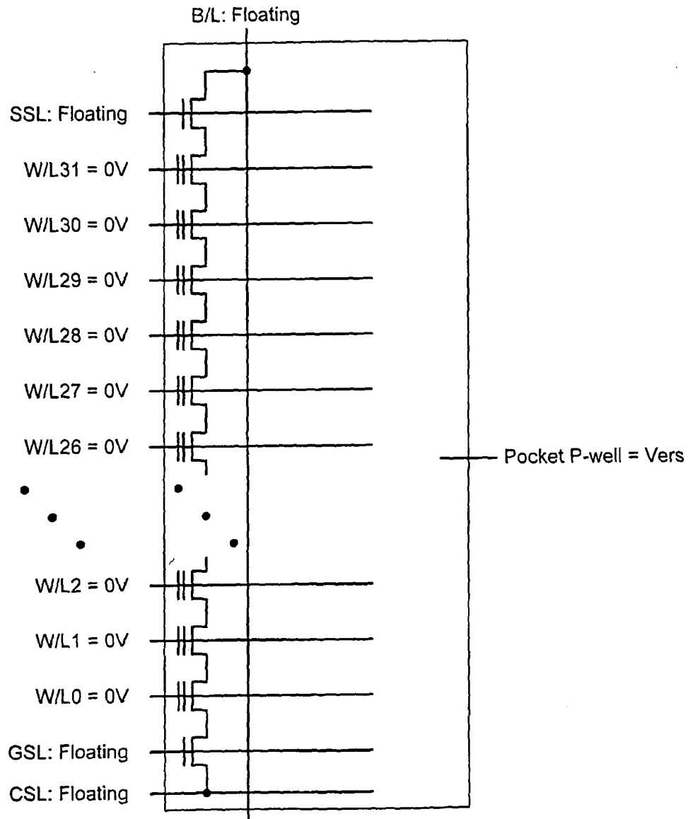
Fig. 14 Prior Art
