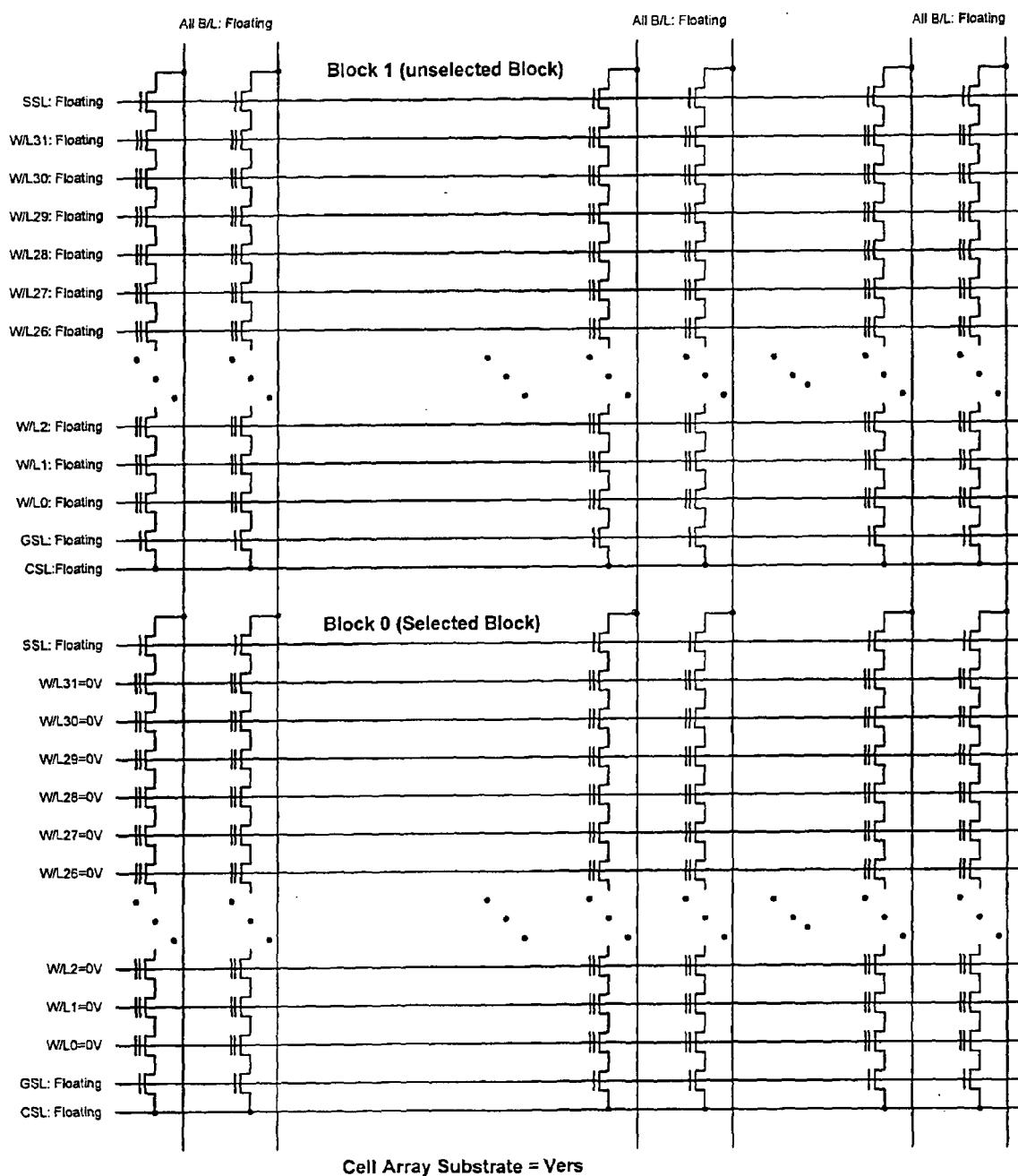
Fig. 15 Prior Art
