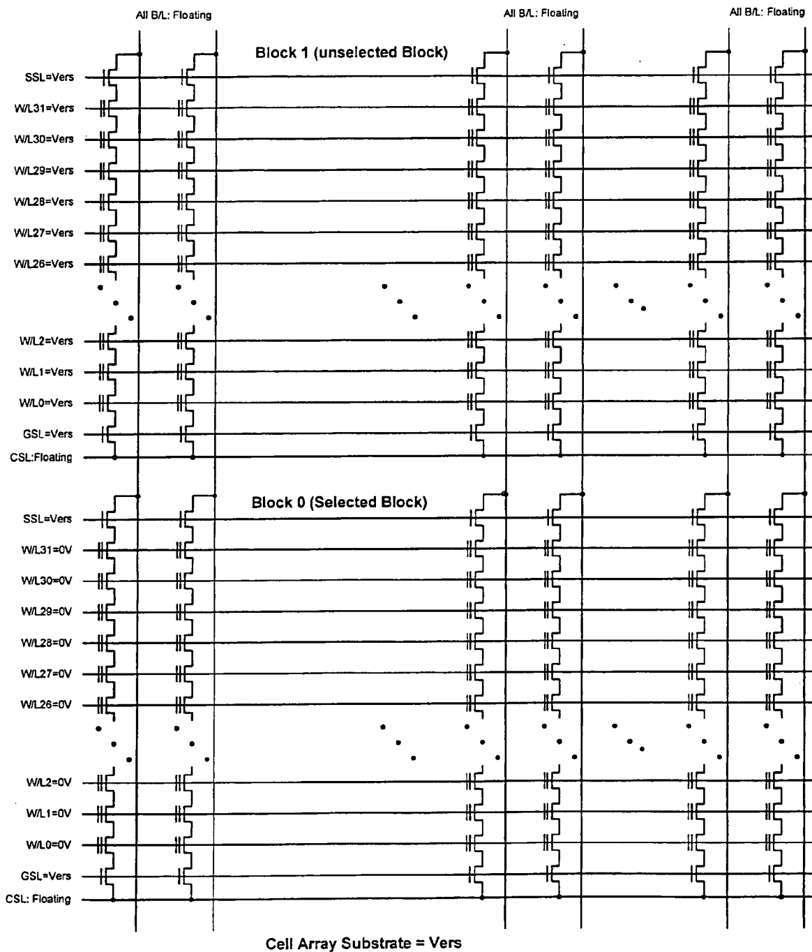
Fig. 13 Prior Art
