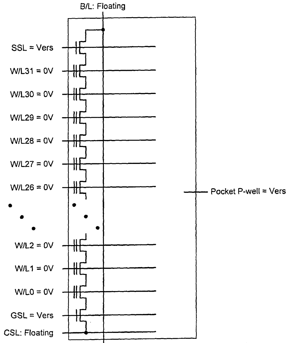
Fig. 12 Prior Art
