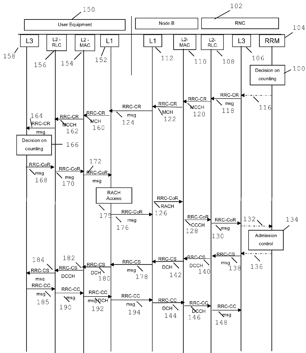
FIG. 1 - PRIOR ART
