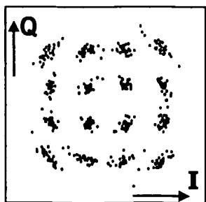
CASE WHERE NOISE IS ADDED IN FIG. 7D TO OBTAIN DELAY AMOUNT OF OPTICAL DELAY DETECTOR T=1.05/R_b
