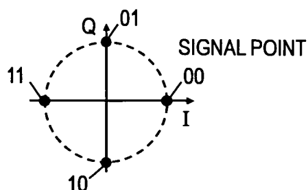
FOUR-LEVEL PHASE MODULATION (QPSK)
