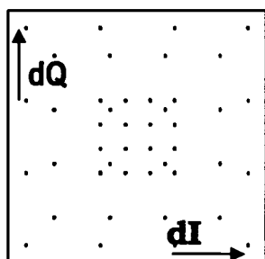
QUADRATURE DELAY DETECTION SIGNAL (dI,dQ) OF FIG. 7B
