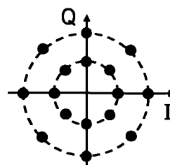
SIXTEEN-LEVEL PHASE AND AMPLITUDE MODULATION (16APSK)
