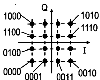
SIXTEEN-LEVEL QUADRATURE AMPLITUDE MODULATION (16QAM)
