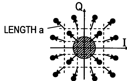
16QAM SIGNAL AFTER AMPLITUDE CONVERSION
