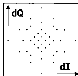
TWO-DIMENSIONAL DISPLAY OF OUTPUTS (X,Y) FROM DELAY DETECTOR ON (dI,dQ)
