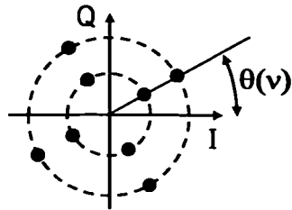
EIGHT-LEVEL PHASE AND AMPLITUDE MODULATION (8-APSK) (CONVENTIONAL TECHNOLOGY)
