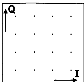
16QAM SIGNAL TO BE TRANSMITTED
