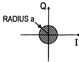
PROHIBITED AREA OF COMPLEX SIGNAL
