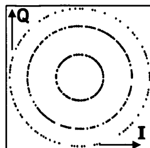
PHASE ACCUMULATION SIGNAL OF FIG. 7A
