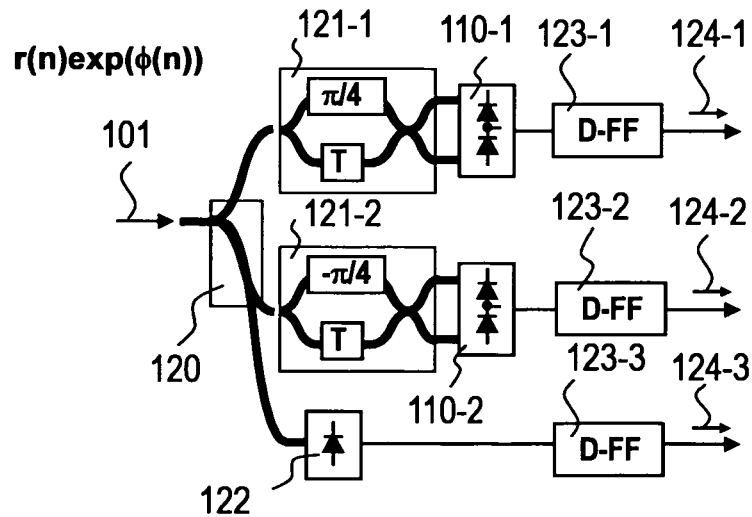
OPTICAL MULTILEVEL SIGNAL RECEIVER FOR RECEIVING 8APSK SIGNAL (CONVENTIONAL TECHNOLOGY)
