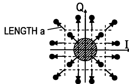
16QAM SIGNAL AFTER DIFFERENT AMPLITUDE CONVERSION
