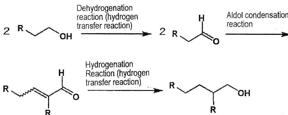
Reaction Scheme 1
