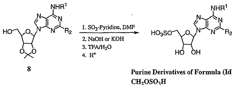
Scheme 6
