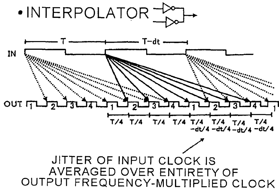
FIG . 13(a) DIRECT CLOCK-CYCLE INTERNAL-DIVISION METHOD
