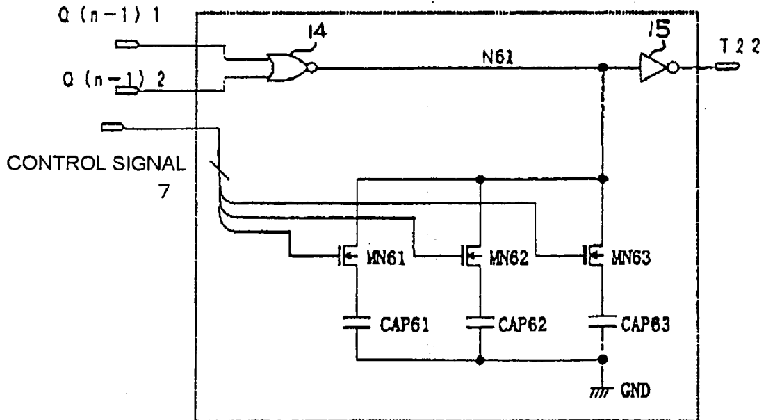
TIMING-DIFFERENCE DIVIDING CIRCUIT 4a2
