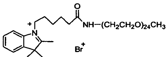
Compound No. 42
