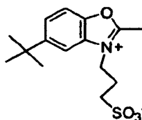
Compound No. 49
