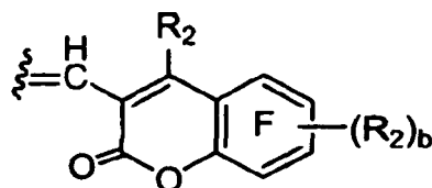
Formula 4
