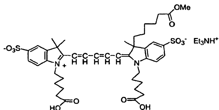
Compound No. 20
