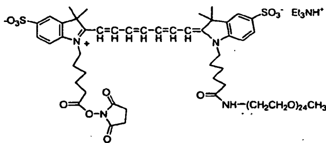
Compound No. 61
