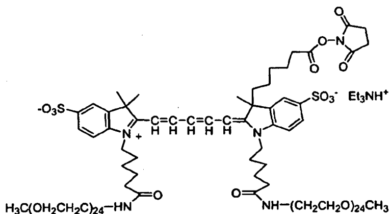
Compound No. 23
