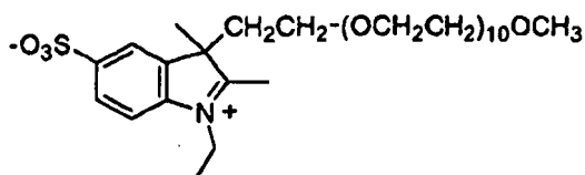
Compound No. 29
