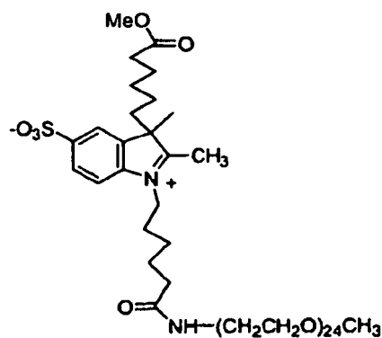
Compound No. 57
