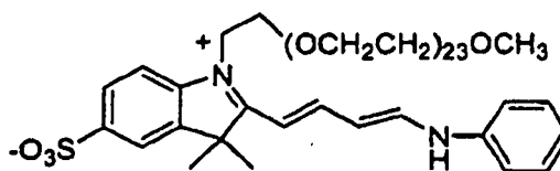
Compound No. 39
