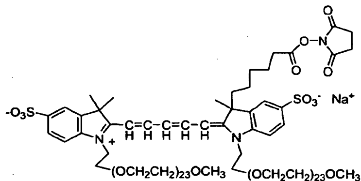
Compound No. 41
