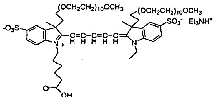
Compound No. 35
