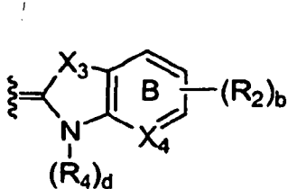
Formula 1
