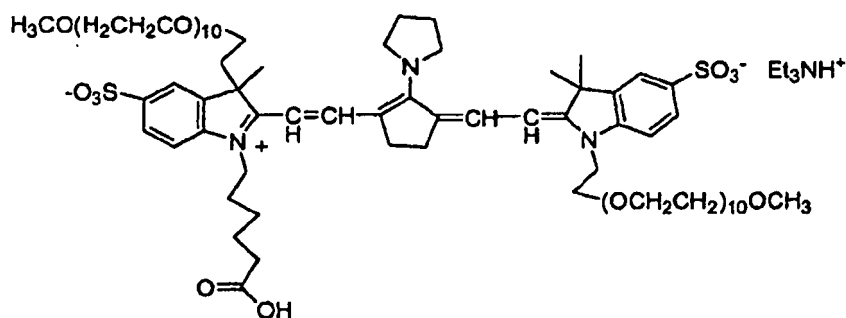
Compound No. 71
