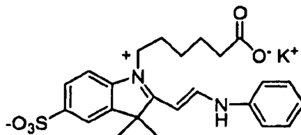
Compound No. 1
