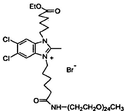
Compound No. 48
