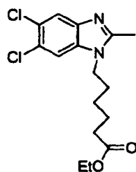
Compound No. 46
