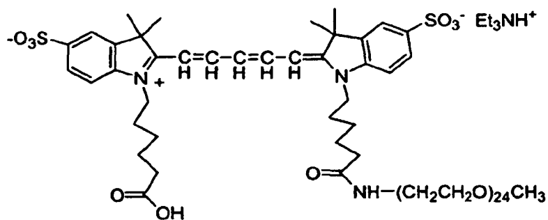
Compound No. 6
