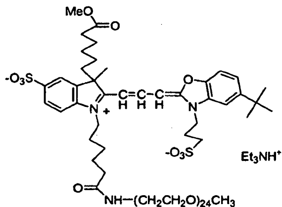
Compound No. 58
