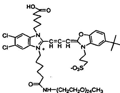
Compound No. 51
