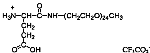
Compound No. 74
