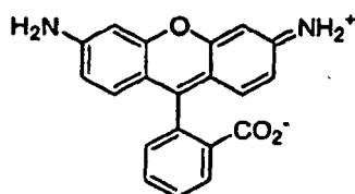
Formula C
