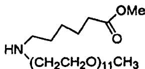
Compound No. 89
