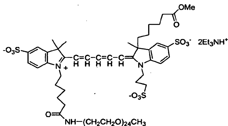
Compound No. 16
