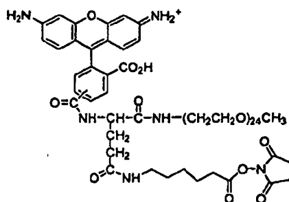
Compound No. 77
