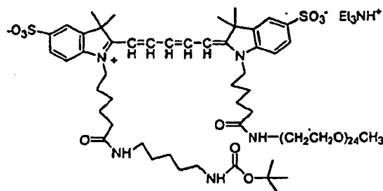
Compound No. 87
