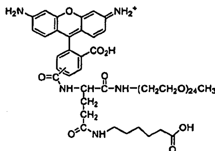
Compound No. 76
