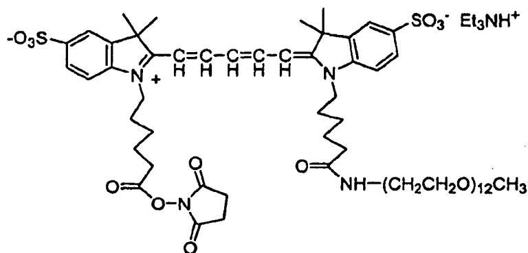
Compound No. 9
