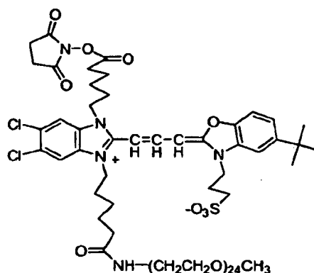
Compound No. 52
