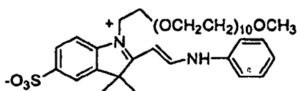
Compound No. 70
