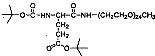
Compound No. 73
