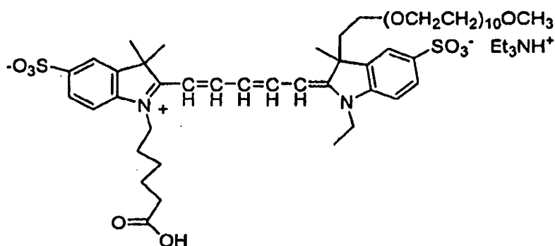
Compound No. 30
