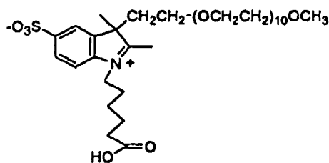
Compound No. 31
