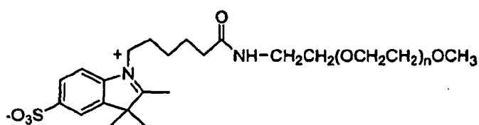
Compound No. 10
