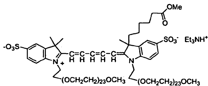
Compound No. 40
