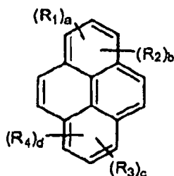
Formula V
