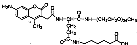
Compound No. 79
