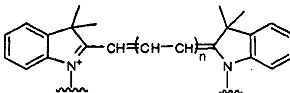
Formula D
