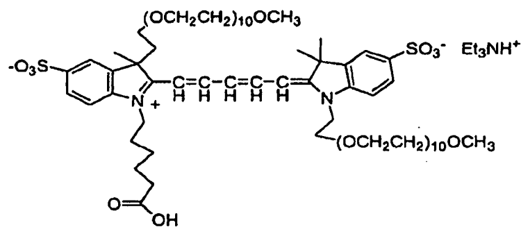
Compound No. 37
