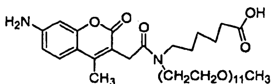
Compound No. 91
