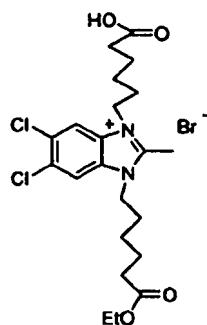
Compound No. 47
