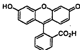
Formula B
