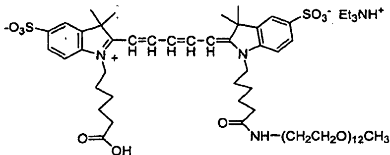
Compound No. 8
