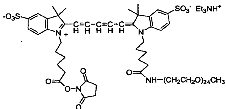
Compound No. 7
