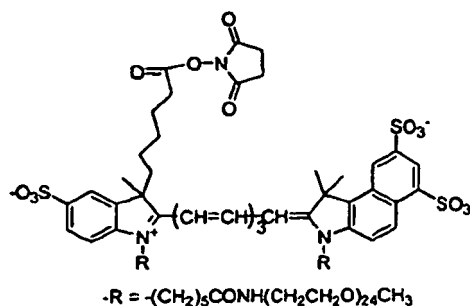
Dye 31
