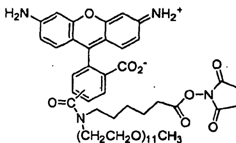
Compound No. 96
