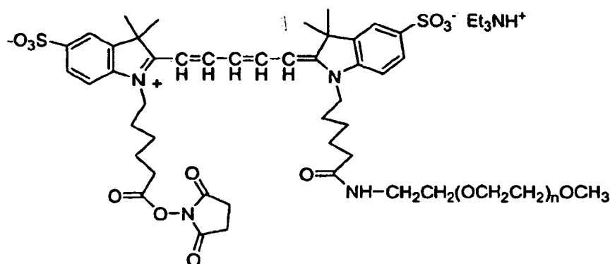
Compound No. 12
