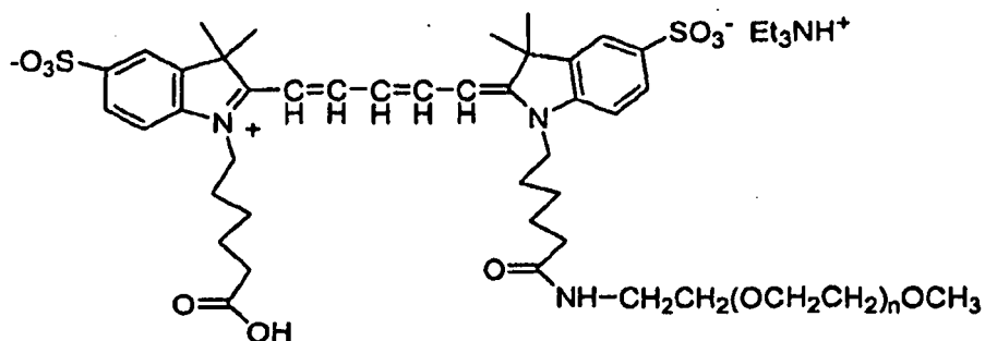
Compound No. 11
