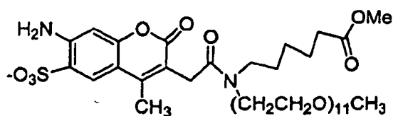
Compound No. 93
