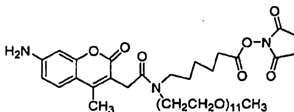
Compound No. 92
