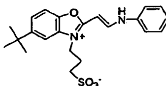
Compound No. 50
