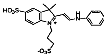
Compound No. 54
