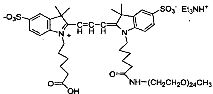
Compound No. 4
