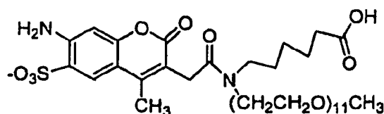
Compound No. 94
