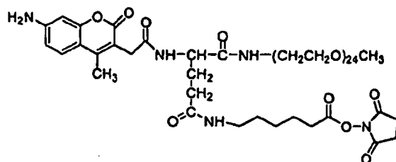
Compound No. 80
