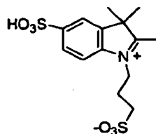
Compound No. 53
