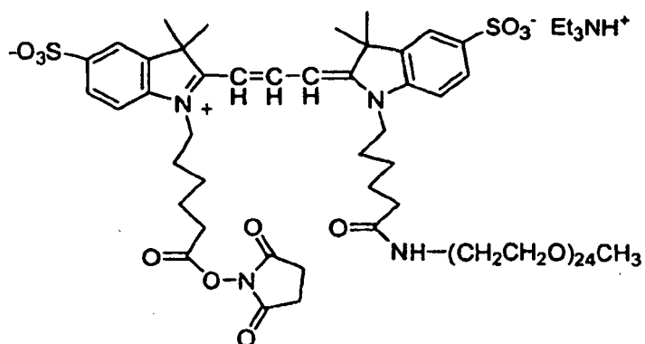
Compound No. 5
