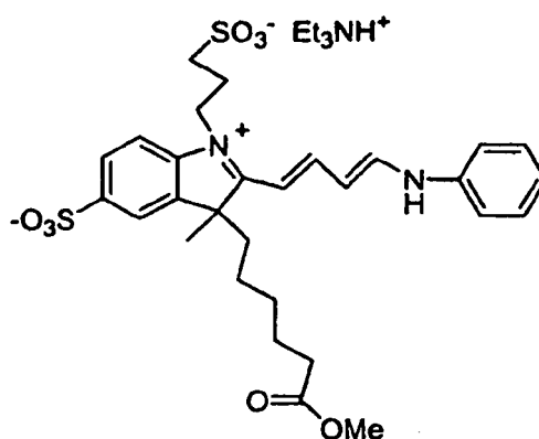
Compound No. 15
