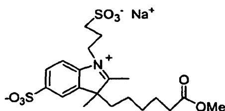
Compound No. 14
