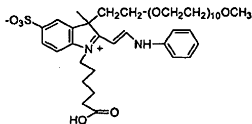
Compound No. 69
