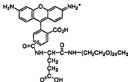
Compound No. 75
