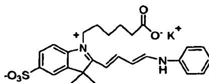
Compound No. 2
