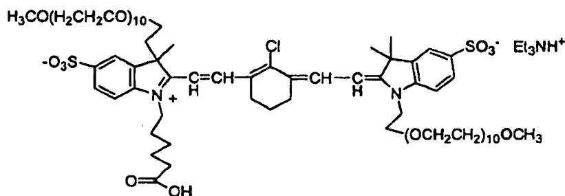
Compound No. 72
