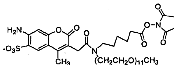
Compound No. 95
