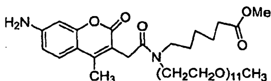
Compound No. 90
