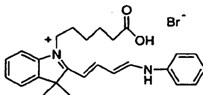
Compound No. 43
