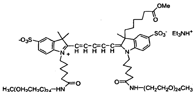
Compound No. 21
