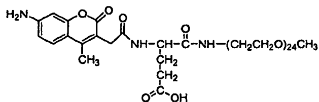
Compound No. 78
