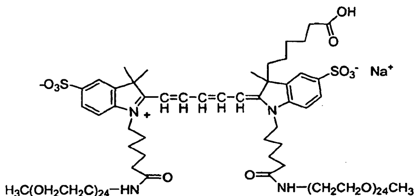
Compound No. 22
