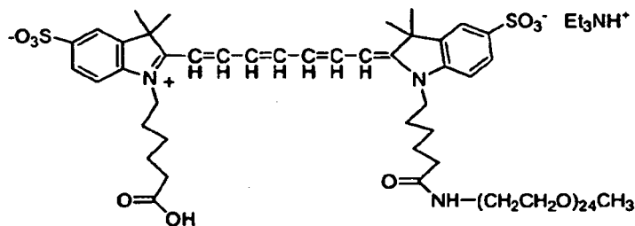
Compound No. 60
