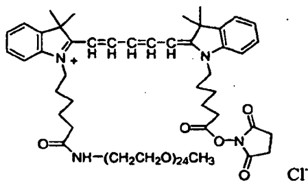
Compound No. 45
