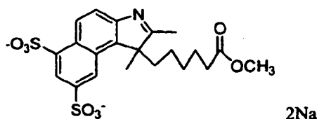
Compound No. 62
