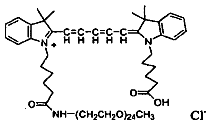
Compound No. 44
