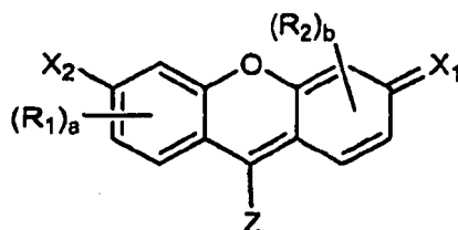
Formula III
