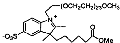
Compound No. 38.
