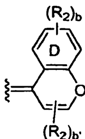
Formula 2
