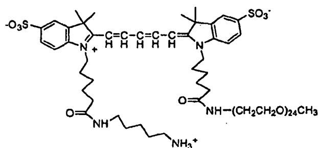
Compound No. 88
