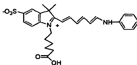
Compound No. 59
