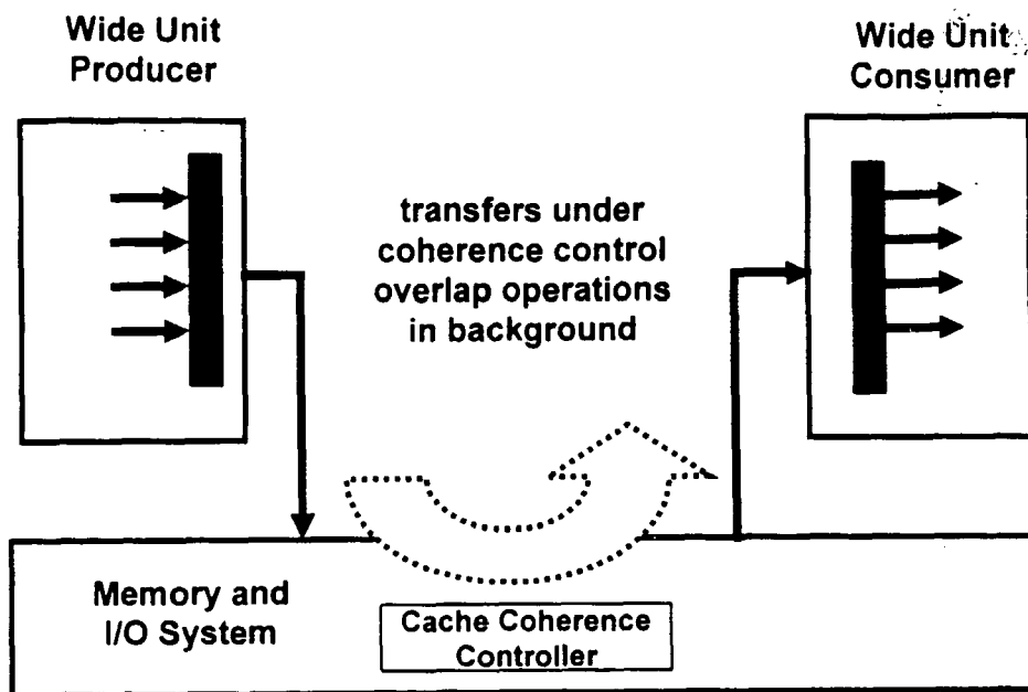
Figure 38 Wide Embedded Cache Coherency
