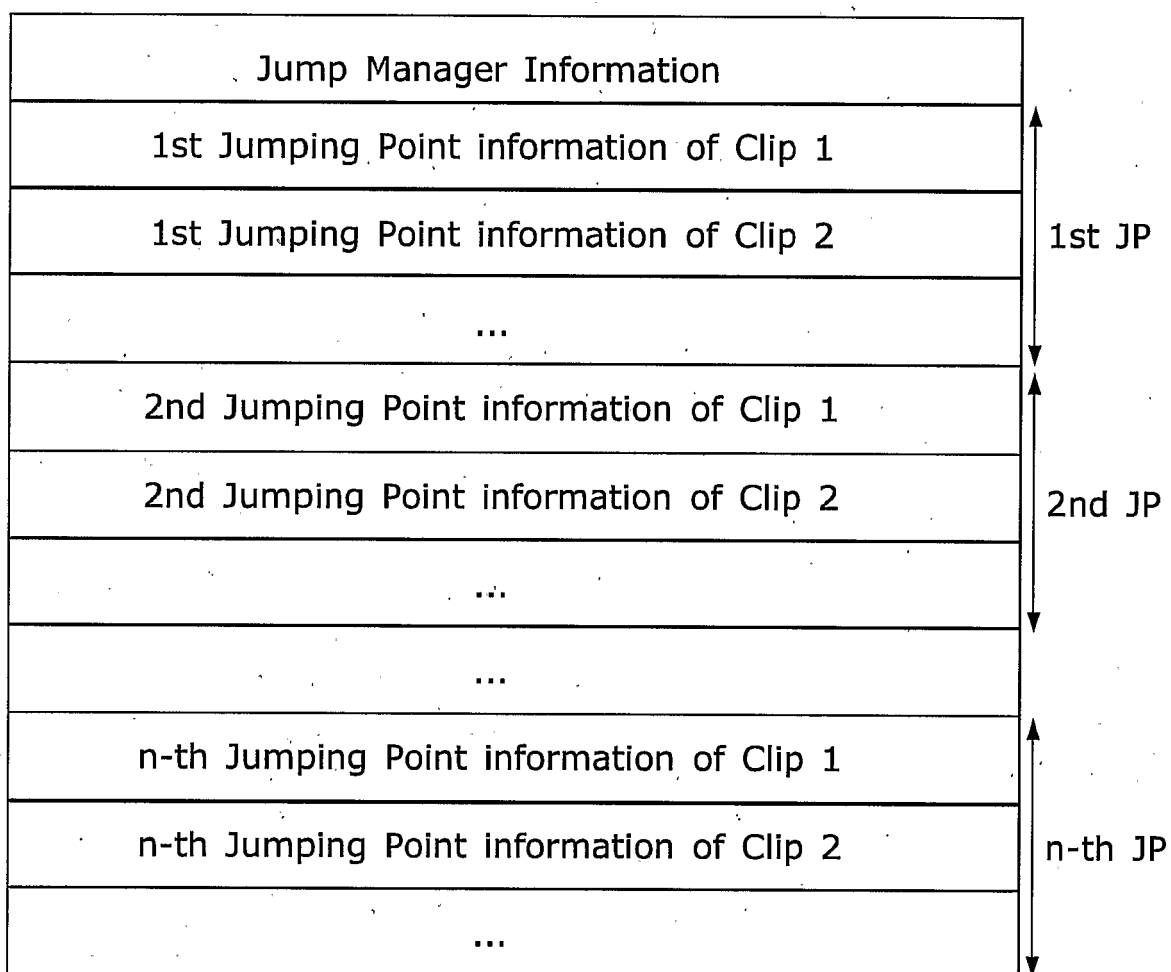
FIG. 19 Jumping Point Map Information
