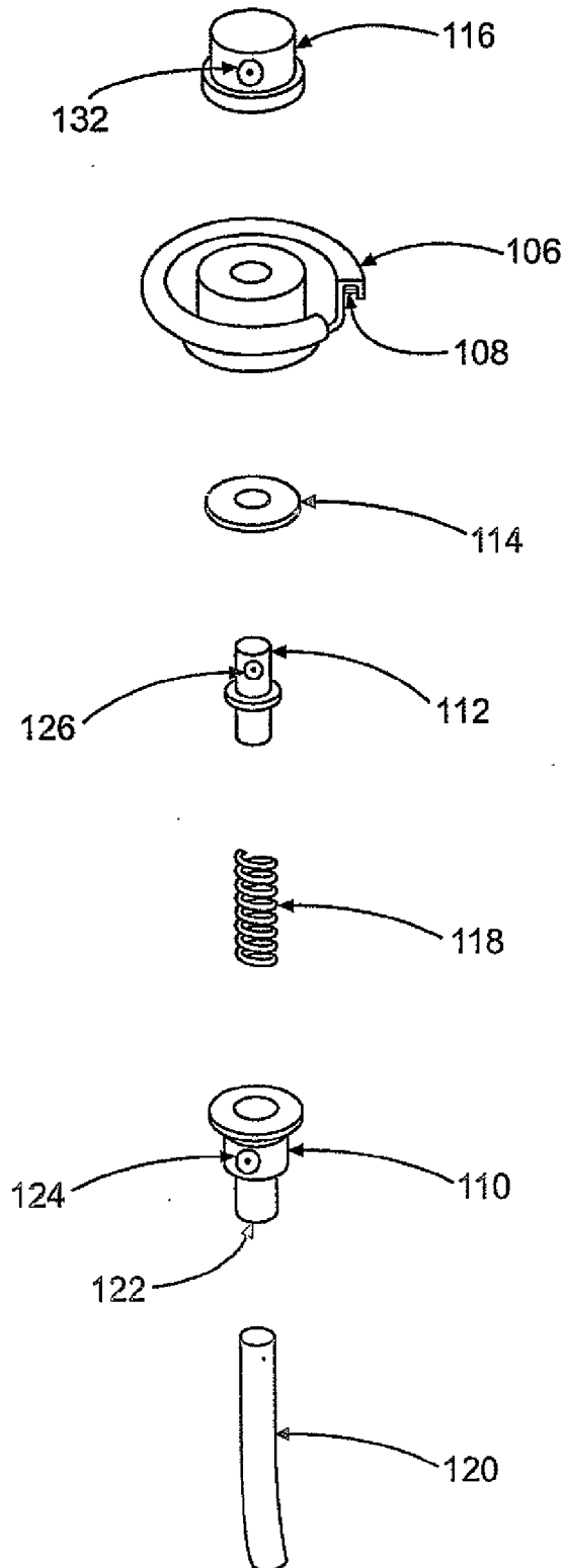
FIG. 3 PRIOR ART
